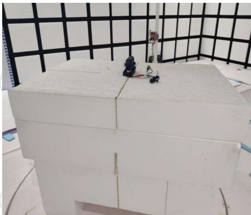
Radiated spurious emission Test Setup-2(Above 1GHz)
