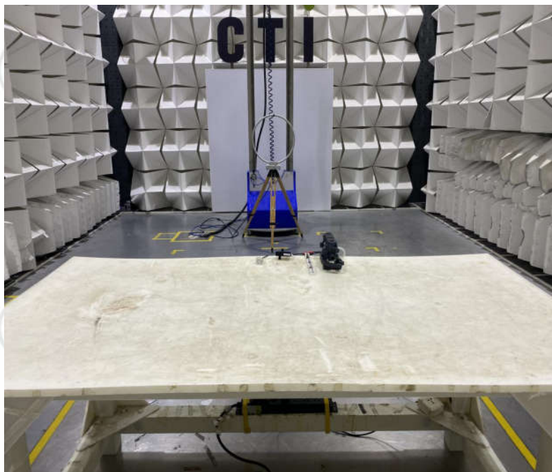
Radiated spurious emission Test Setup-1(Below 30MHz)
