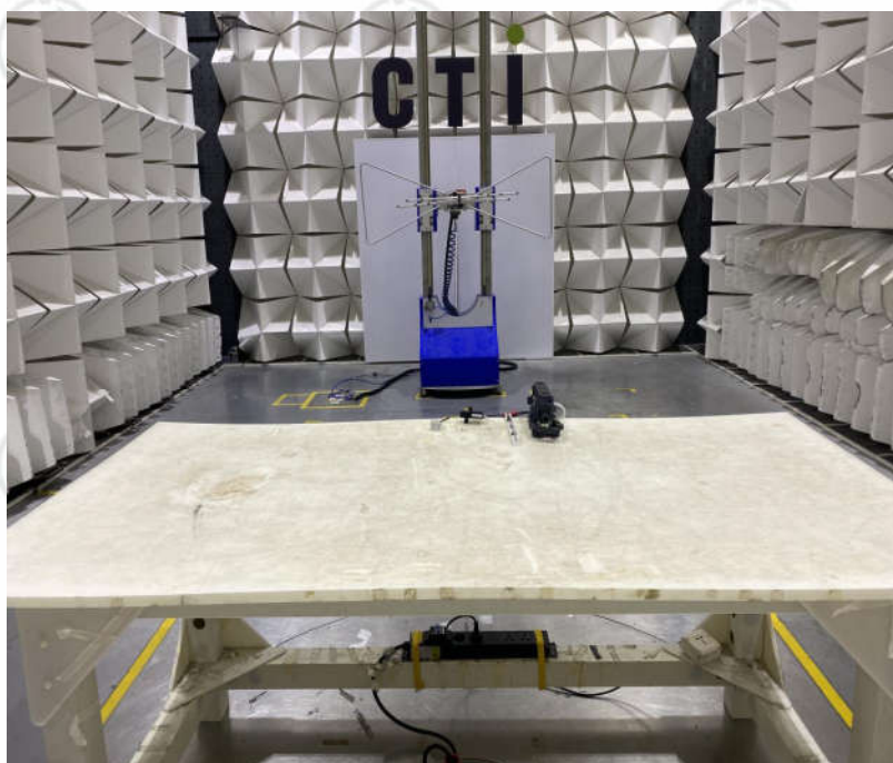
Radiated spurious emission Test Setup-1(Below 1GHz)
