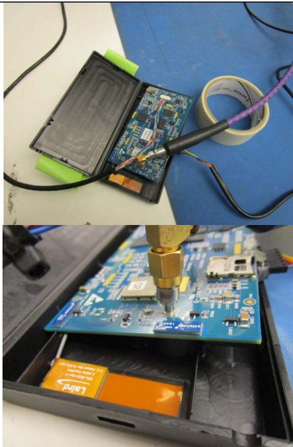
Conducted RF Test Setup
