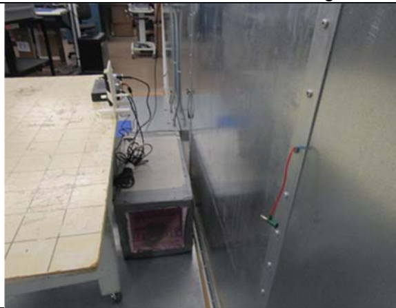
Conducted AC Mains Testing
