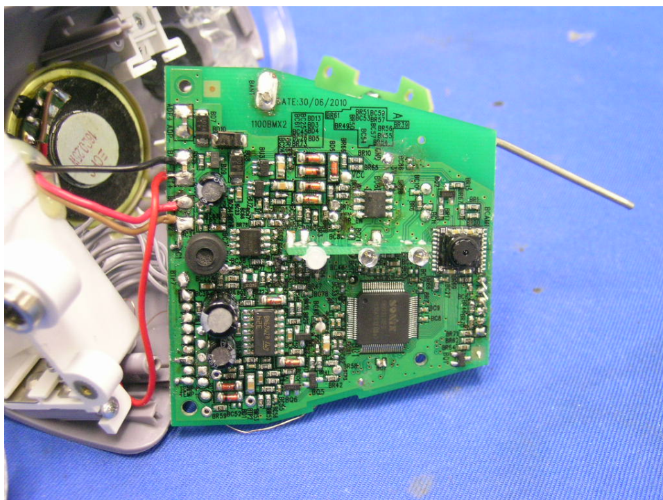
Baby Unit Main PCB comp side (View 1)
