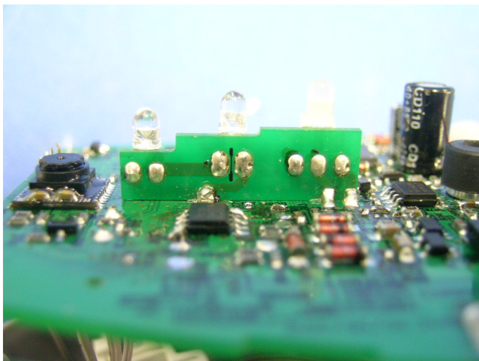
Baby Unit Main PCB comp side (View 3)
