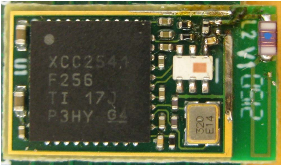
Front side of module
