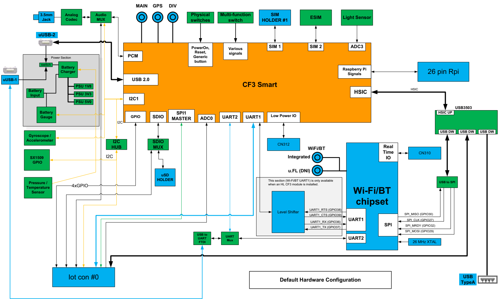
Figure 2-4: mangOH Red Hardware Architecture (Default)
