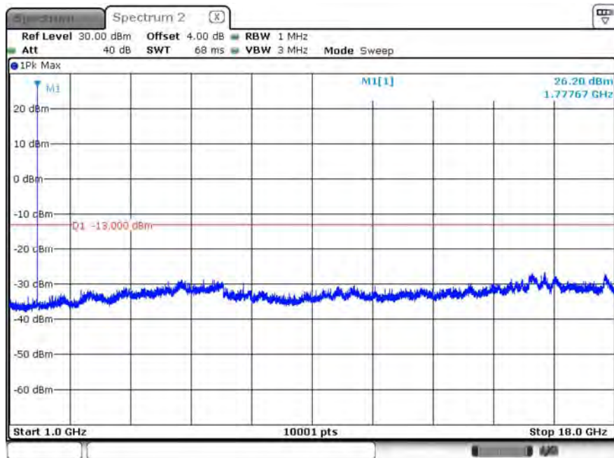
B66_CH132647_5M_1RB12_16-QAM_Above 1G
