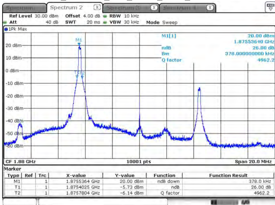
B2_CH18900_10M_QPSK_1RB0_26dB BW
