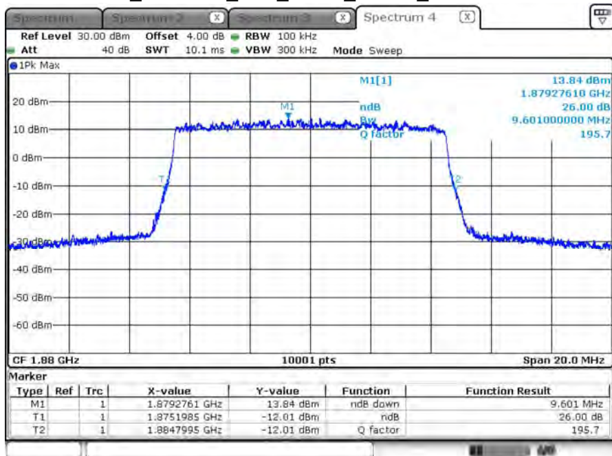
B2_CH18900_10M_QPSK_50RB0_26dB BW
