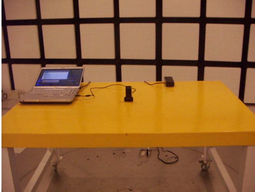
Y-AXIS WITH CRADLE FRONT PHOTO
