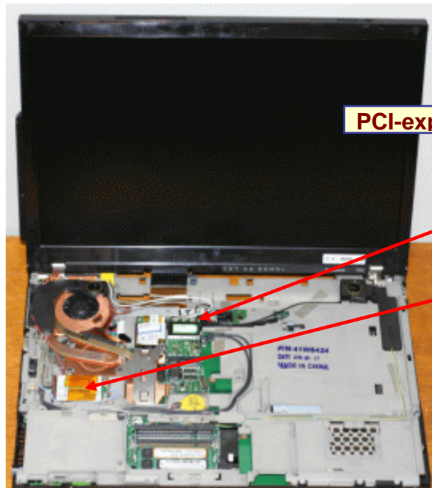
PCI-express WWAN card slot
