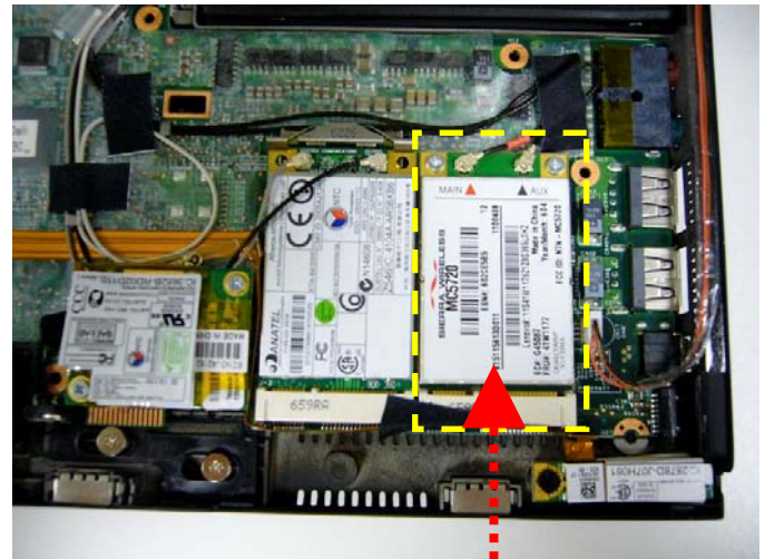
Mini-PCIe Slot for WWAN device
