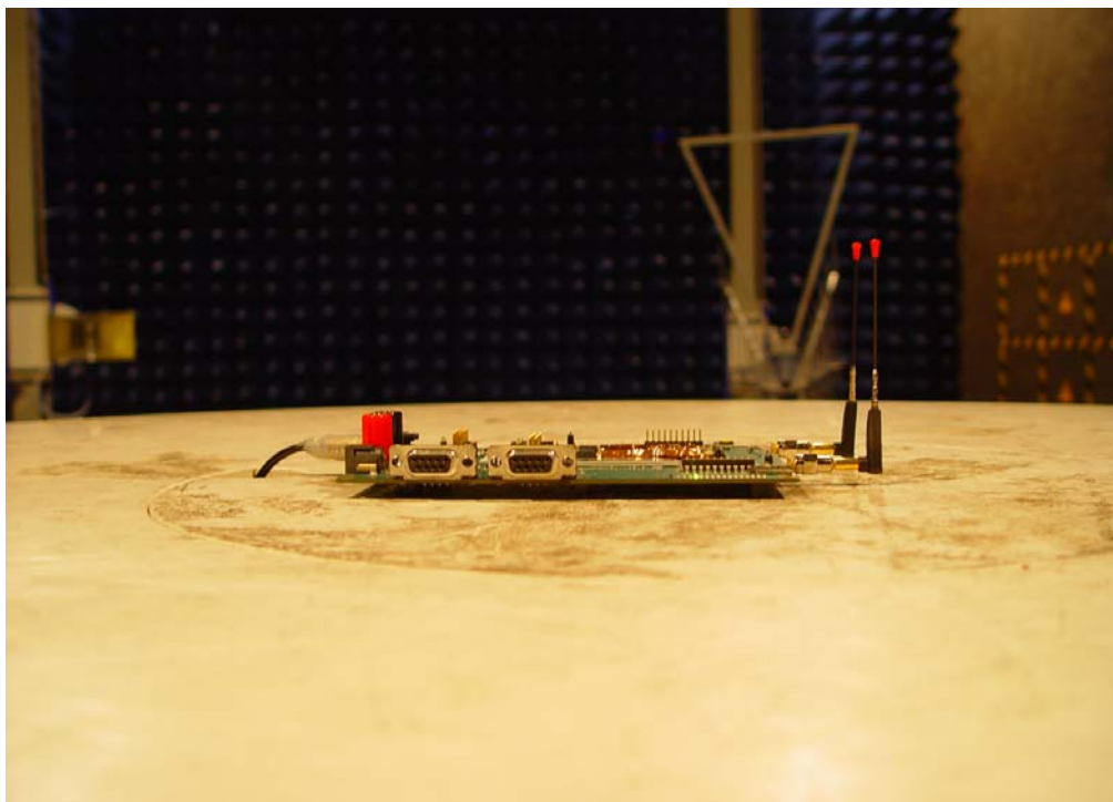
Radiated Spurious Emissions Test setup
