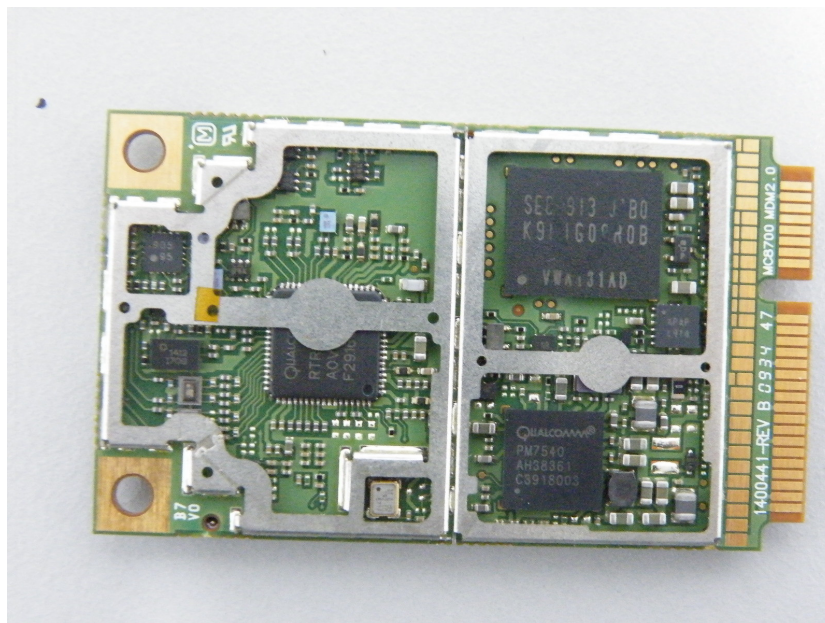
Internal of EUT-1
