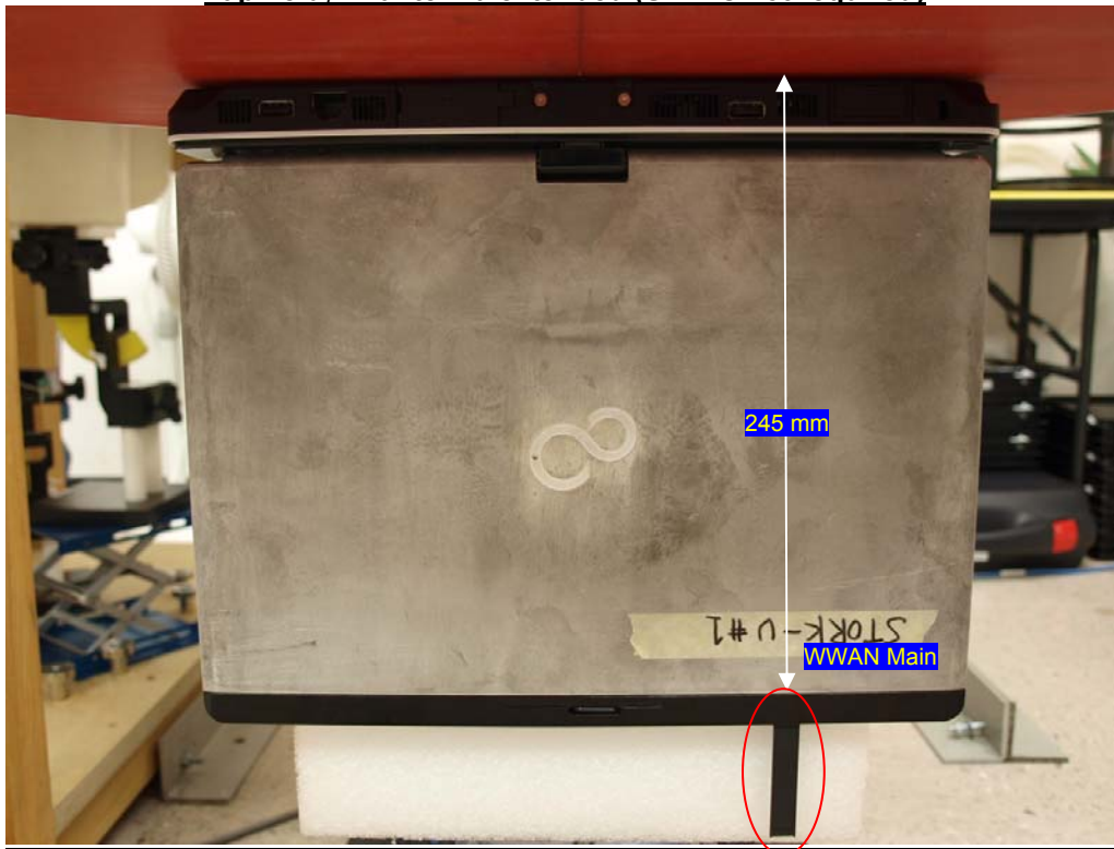
Lap held, w/ antenna extended (SAR is not required)
