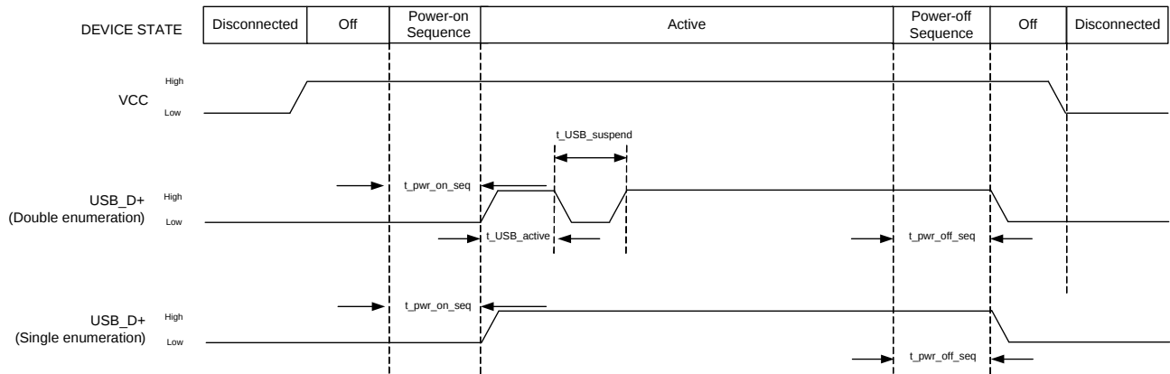
Figure 5-1: Signal Timing (USB Enumeration)
