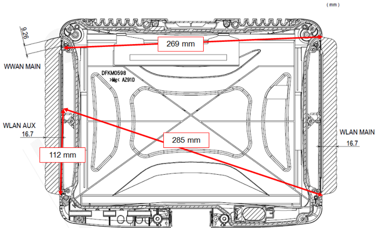
Location of the WWAN main Antenna relative to the indented corners
