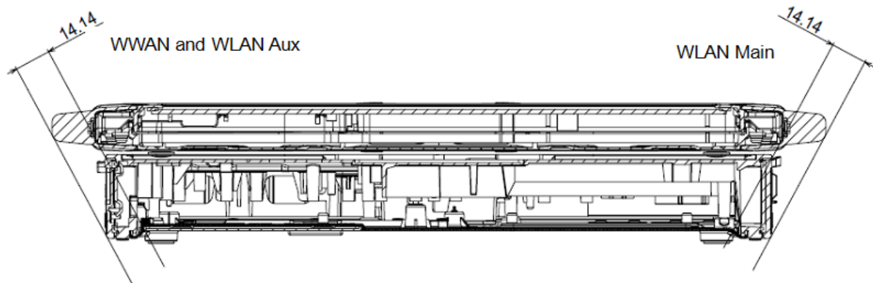
Location of the antennas relative to the protrusions and rear.
