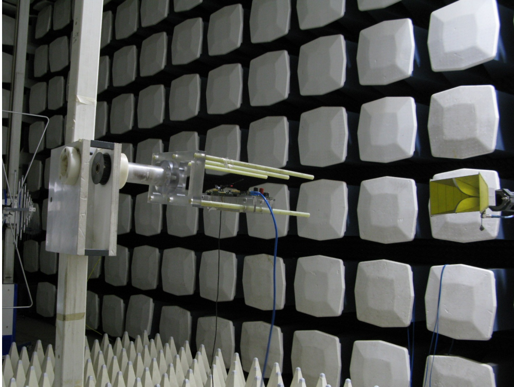
MC7355 Standalone RSE test setup photo
