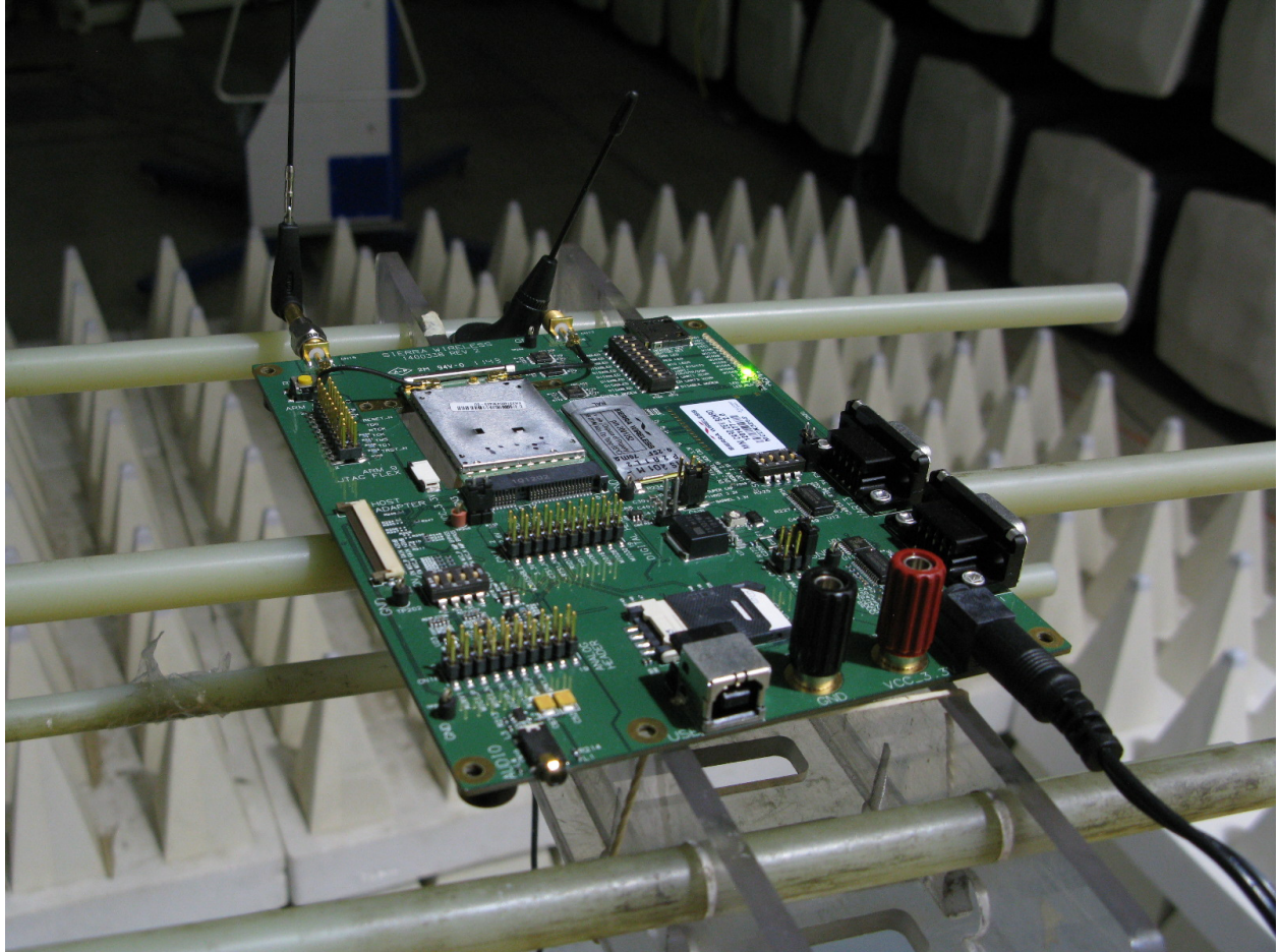
MC7355 standalone RSE test setup photo
