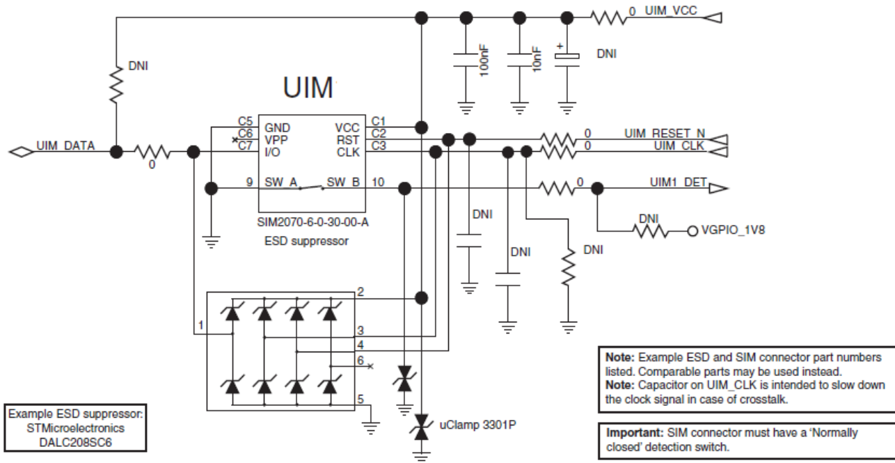
Figure 4-4: UIM Interface
