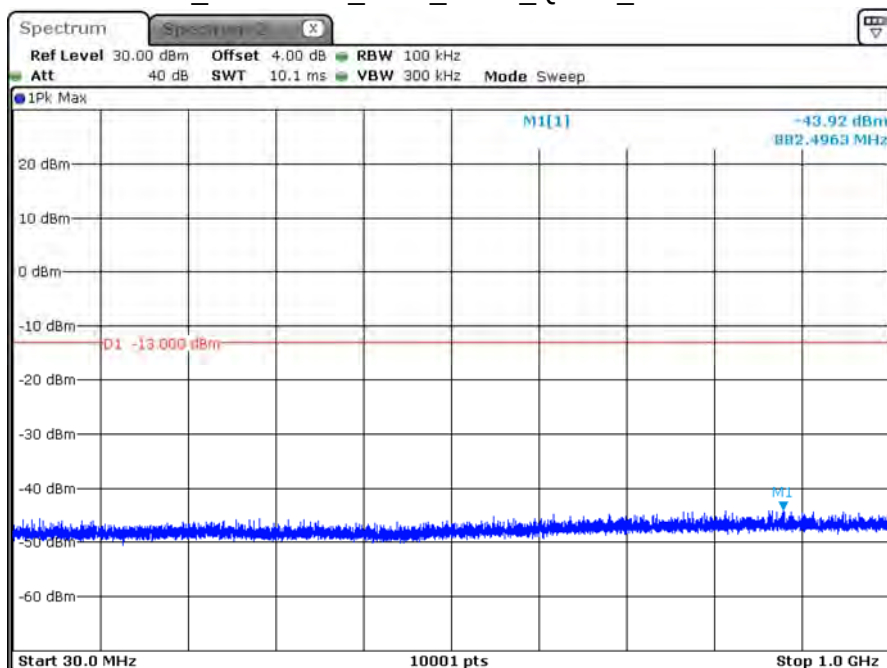
B66_CH131979_1.4M_1RB0_QPSK_Below 1G
