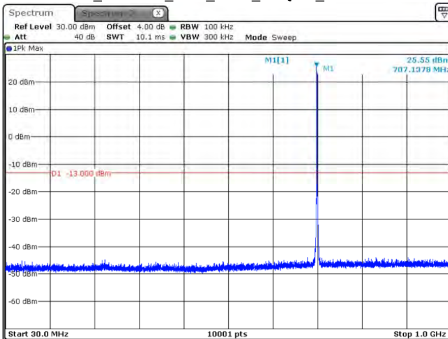
B12_CH23095_1.4M_1RB0_16-QAM_Below 1G
