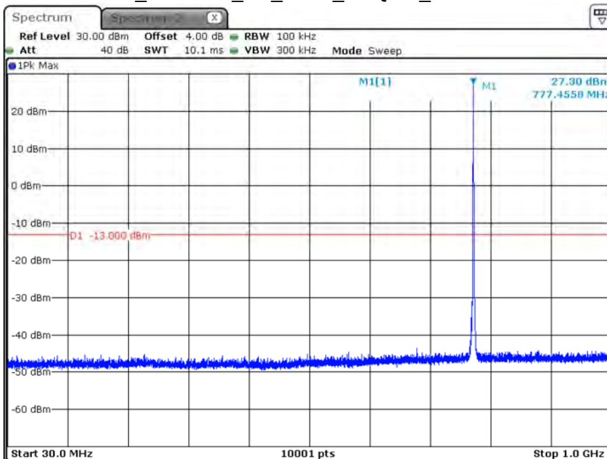
B13_CH23205_5M_1RB0_16-QAM_Below 1G
