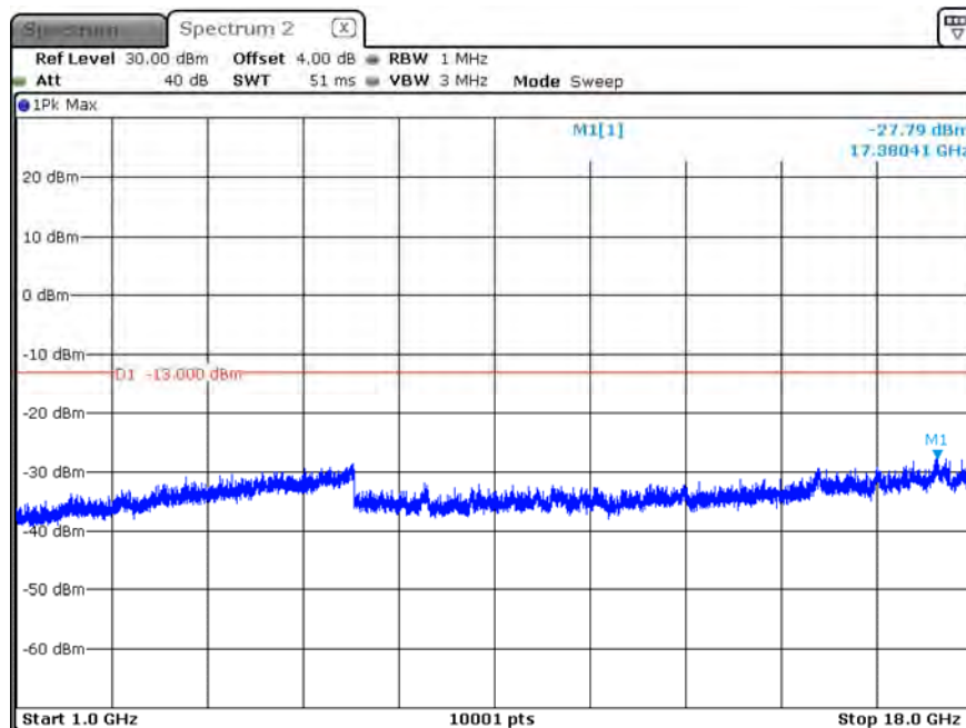
B12_CH23095_3M_1RB0_16-QAM_Above 1G
