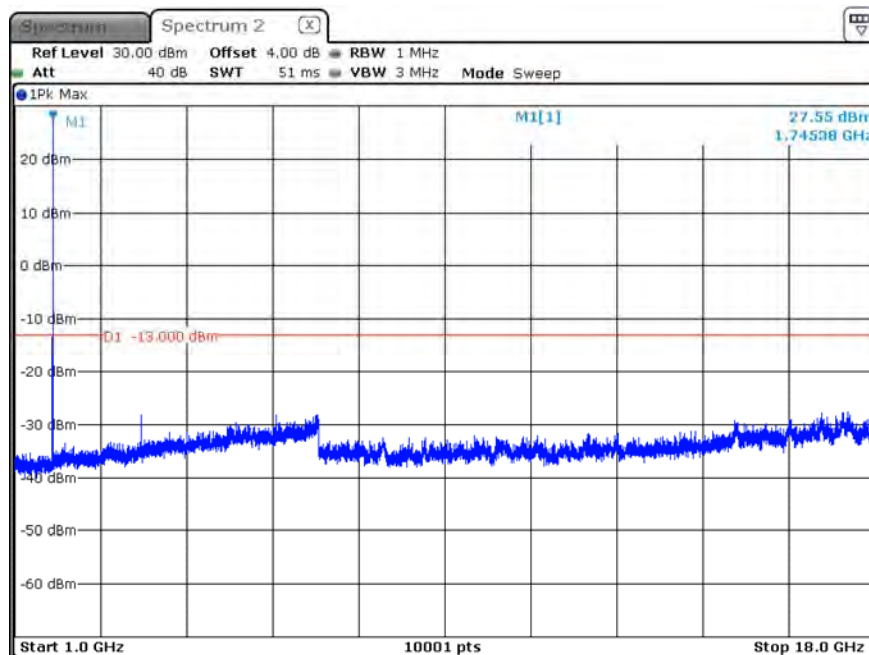
B66_CH132322_1.4M_1RB0_16-QAM_Above 1G
