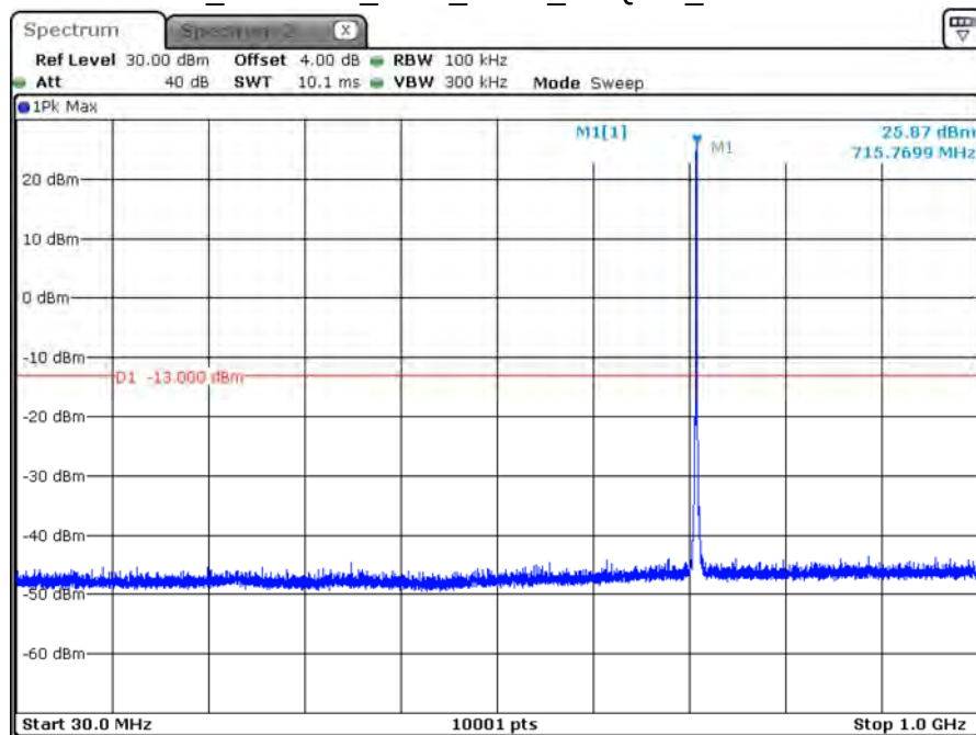
B12_CH23173_1.4M_1RB5_16-QAM_Below 1G
