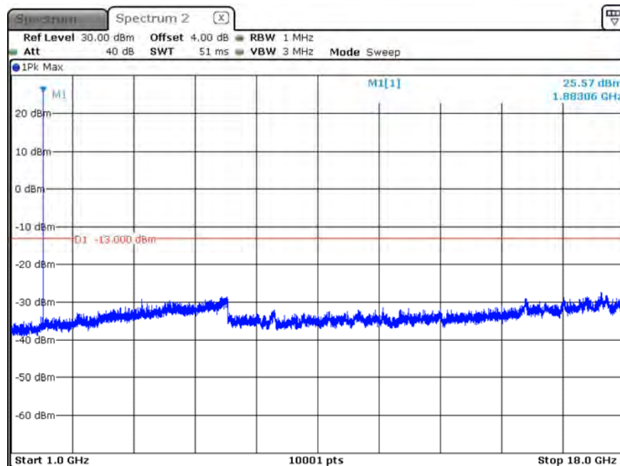
B25_CH26365_1.4M_1RB0_16-QAM_Above 1G
