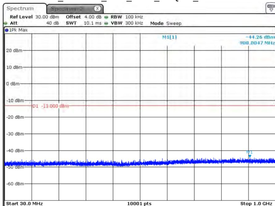
B25_CH26047_1.4M_1RB0_16-QAM_Below 1G
