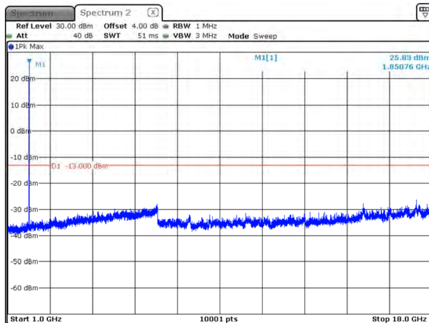
B25_CH26047_1.4M_1RB0_16-QAM_Above 1G
