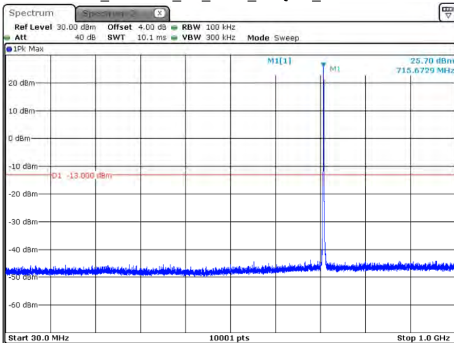
B12_CH23165_3M_1RB5_16-QAM_Below 1G
