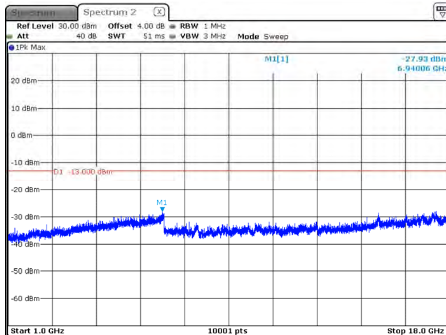
B12_CH23025_3M_1RB0_16-QAM_Above 1G
