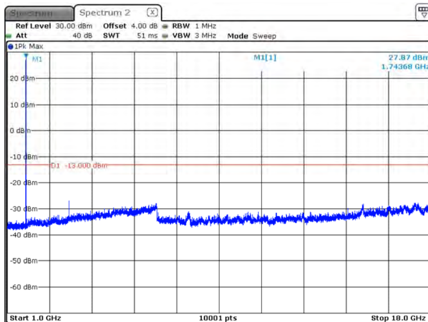
B66_CH132322_5M_1RB0_16-QAM_Above 1G
