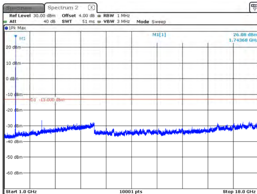
B66_CH132322_3M_1RB0_16-QAM_Above 1G
