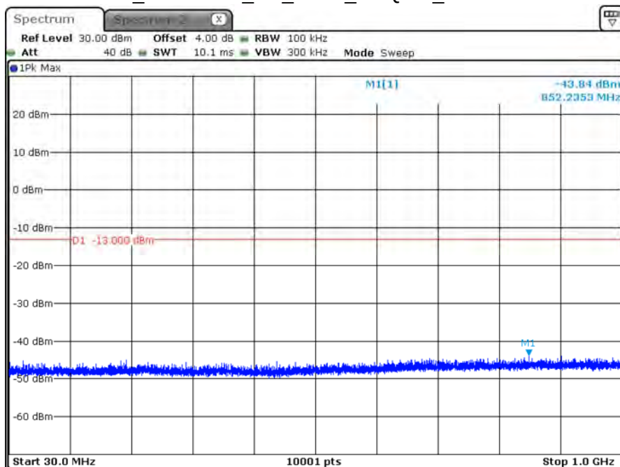
B66_CH132322_5M_1RB0_16-QAM_Below 1G
