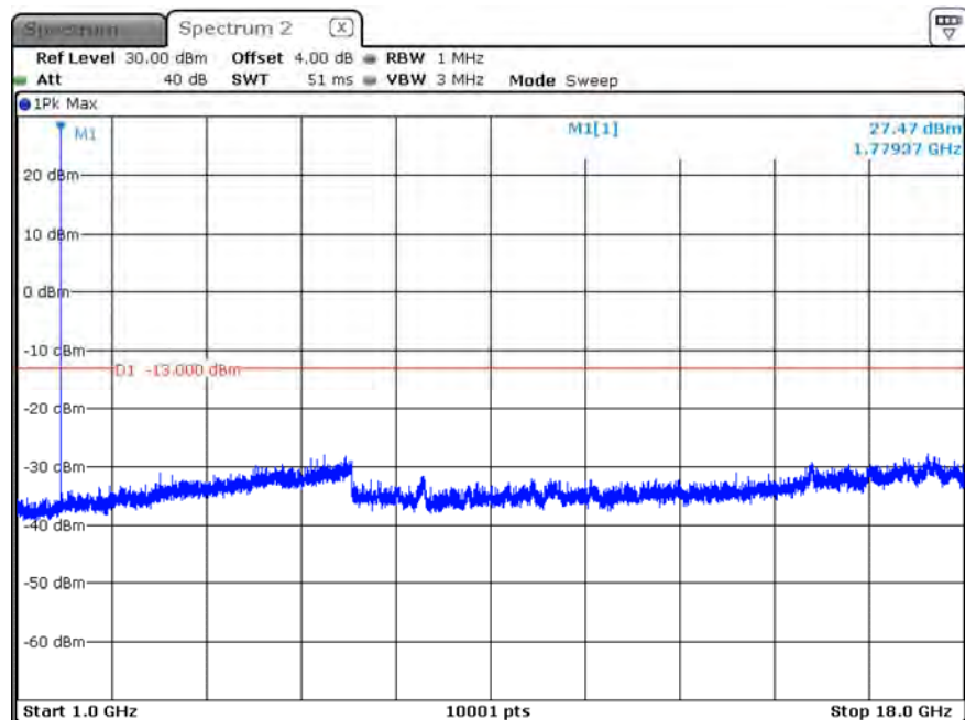
B66_CH132665_1.4M_1RB5_16-QAM_Above 1G
