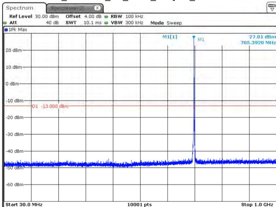
B12_CH23095_5M_1RB0_16-QAM_Below 1G
