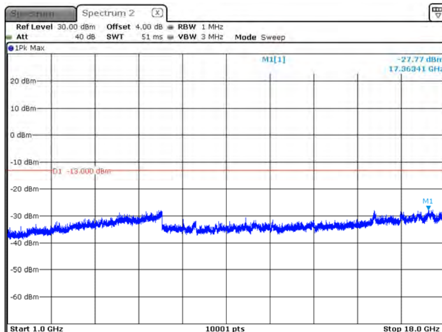
B13_CH23205_5M_1RB0_16-QAM_Above 1G
