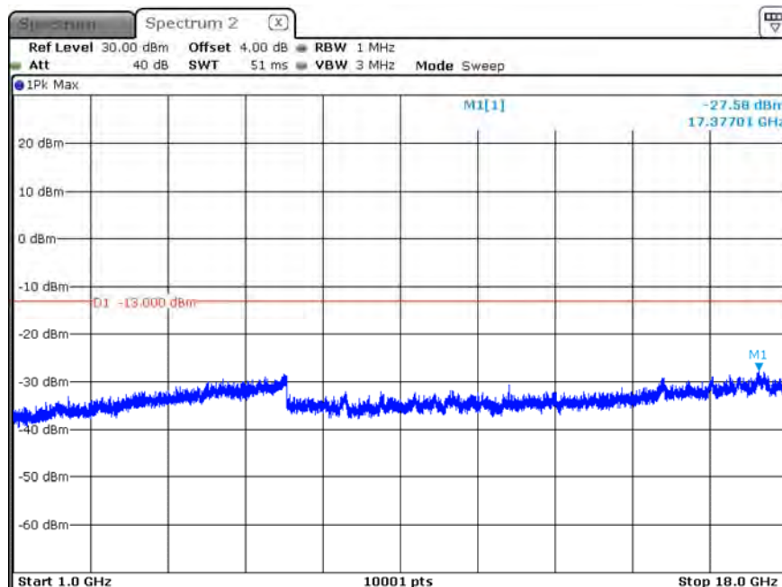
B12_CH23130_10M_1RB5_16-QAM_Above 1G
