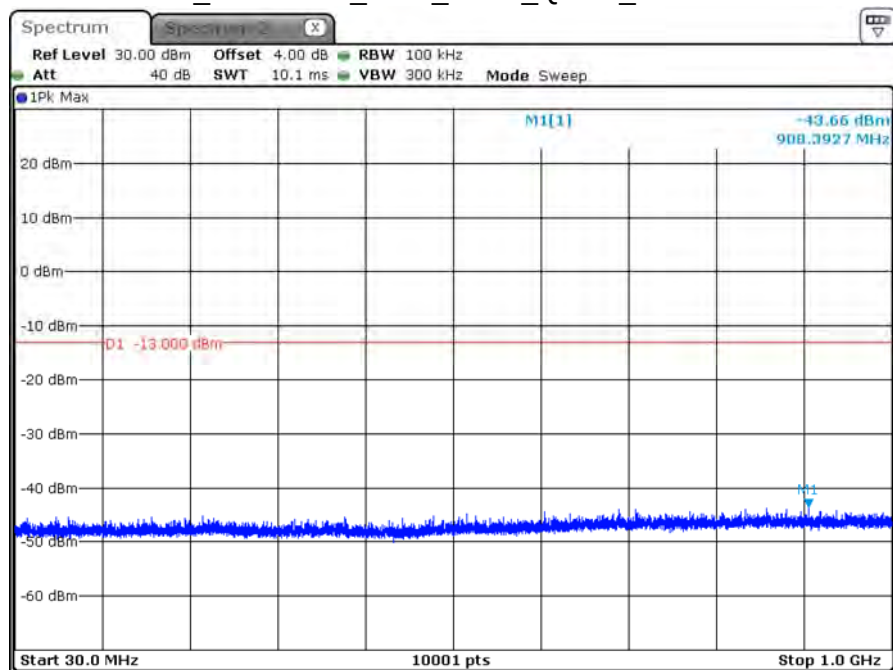
B66_CH132322_1.4M_1RB0_QPSK_Below 1G
