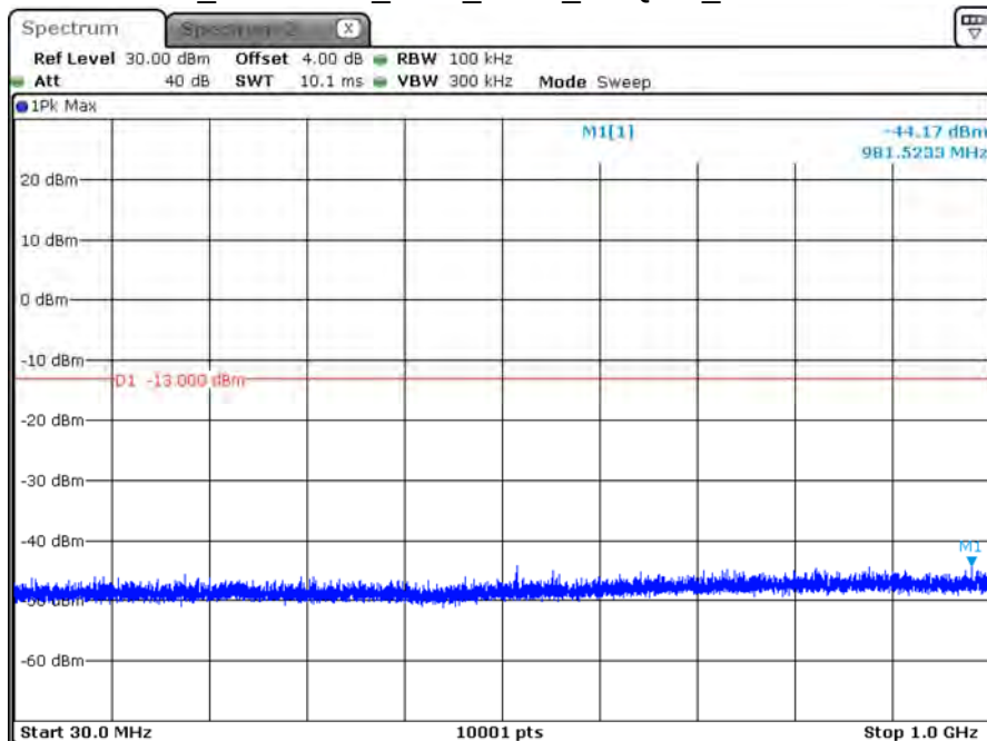
B66_CH132322_1.4M_1RB0_16-QAM_Below 1G
