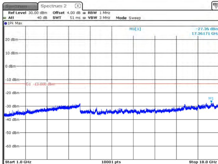
B12_CH23173_1.4M_1RB5_QPSK_Above 1G
