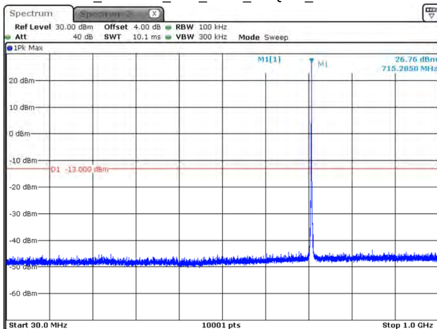
B12_CH23130_10M_1RB5_16-QAM_Below 1G
