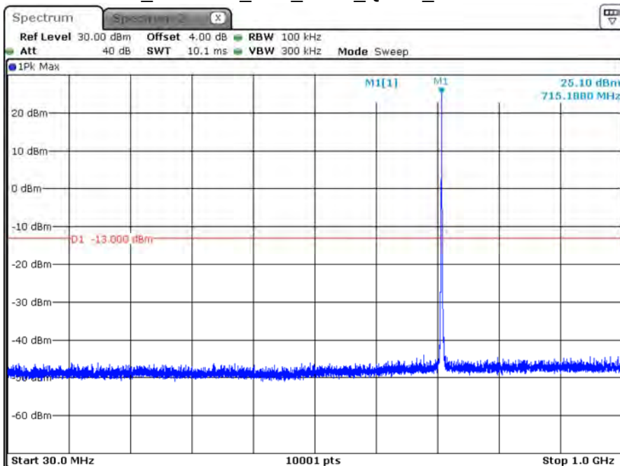
B12_CH23130_10M_1RB5_QPSK_Below 1G
