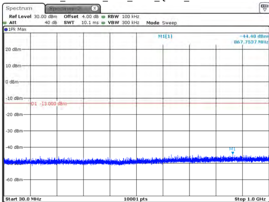
B25_CH26683_1.4M_1RB5_QPSK_Below 1G
