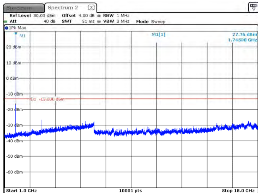
B66_CH132322_1.4M_1RB0_QPSK_Above 1G
