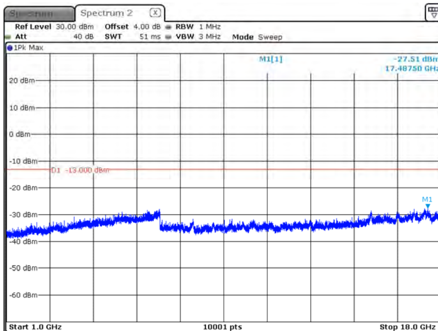
B12_CH23095_1.4M_1RB0_QPSK_Above 1G
