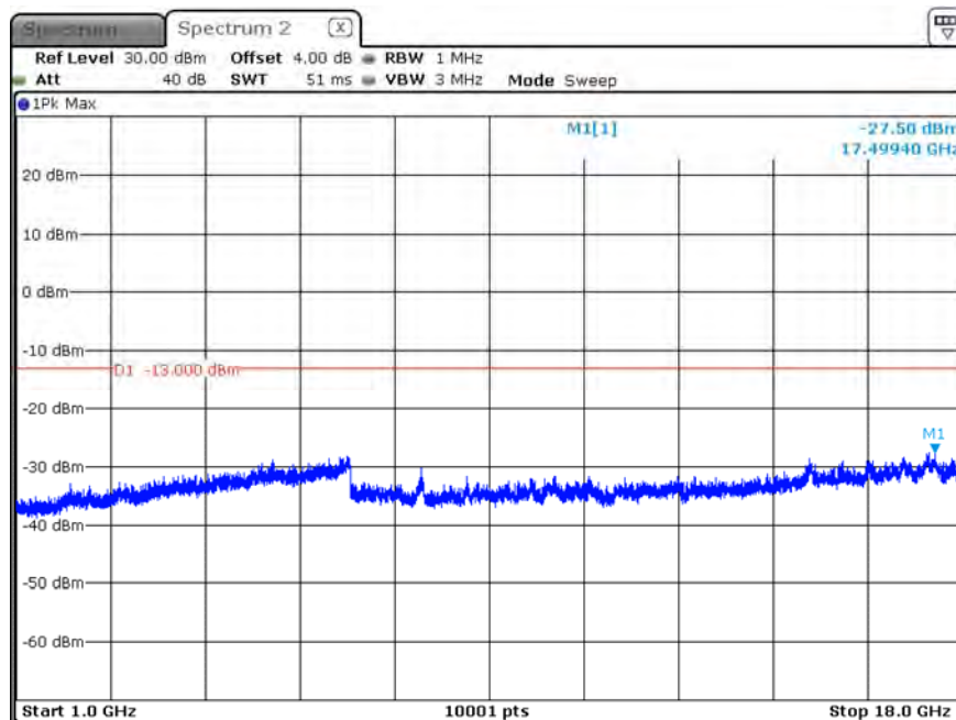
B12_CH23165_3M_1RB5_16-QAM_Above 1G
