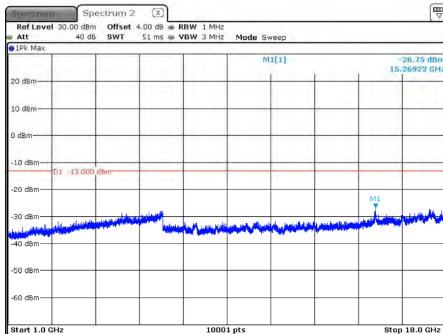
B12_CH23173_1.4M_1RB5_16-QAM_Above 1G
