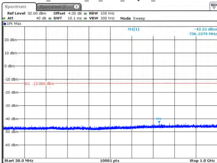
B66_CH132322_3M_1RB0_16-QAM_Below 1G
