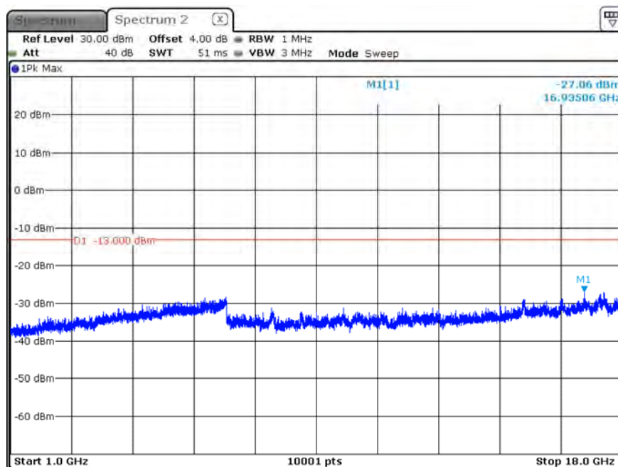
B12_CH23155_5M_1RB5_16-QAM_Above 1G
