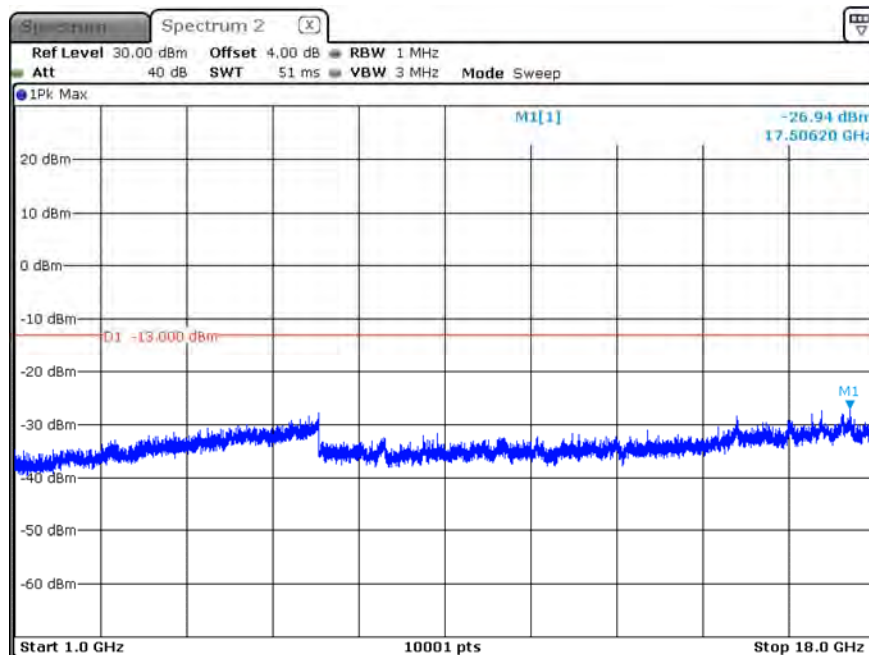
B12_CH23095_5M_1RB0_16-QAM_Above 1G
