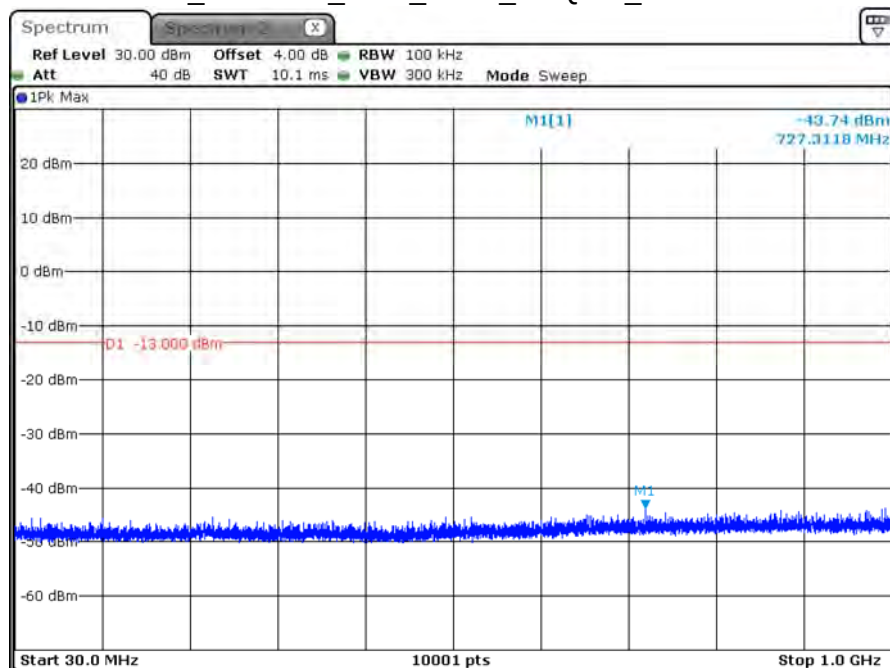
B25_CH26365_1.4M_1RB0_16-QAM_Below 1G
