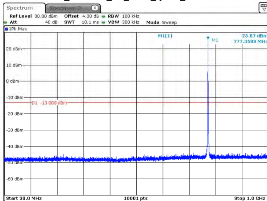
B13_CH23205_5M_1RB0_QPSK_Below 1G
