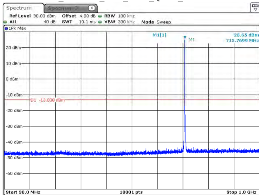
B12_CH23173_1.4M_1RB5_QPSK_Below 1G
