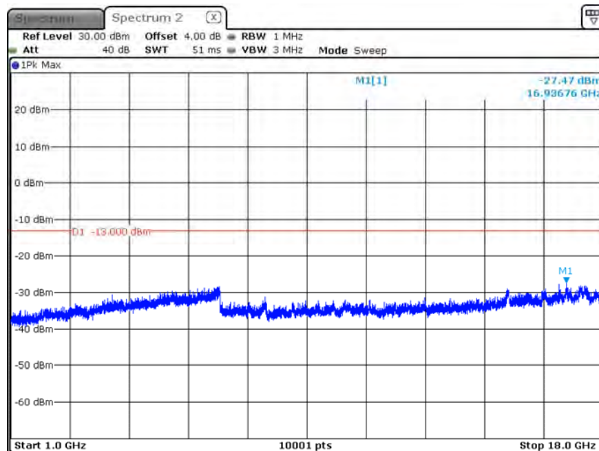
B12_CH23060_10M_1RB0_16-QAM_Above 1G
