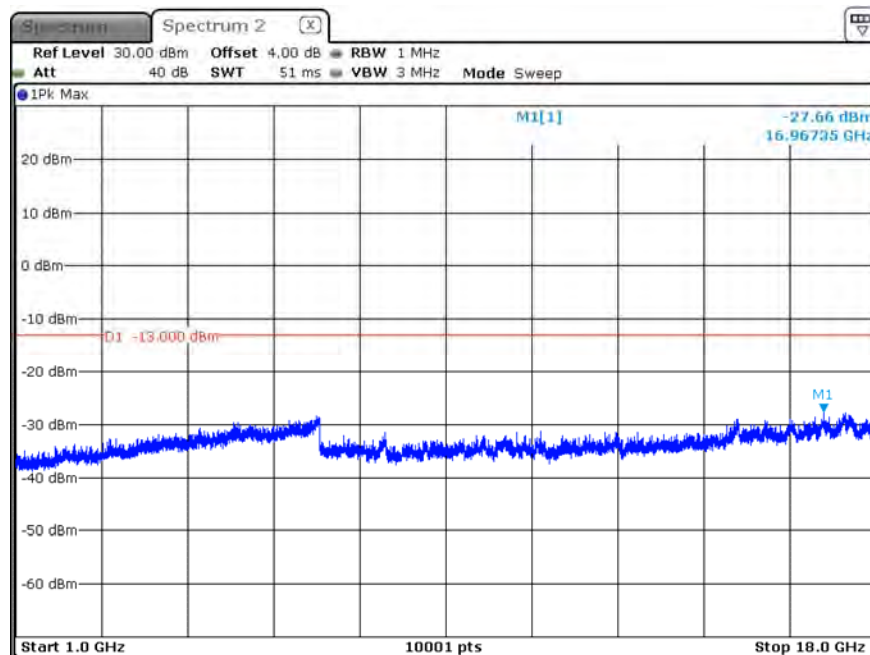
B12_CH23035_5M_1RB0_16-QAM_Above 1G
