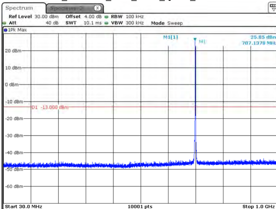
B12_CH23095_1.4M_1RB0_QPSK_Below 1G
