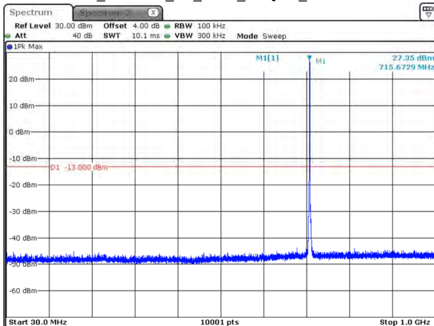
B12_CH23155_5M_1RB5_16-QAM_Below 1G
