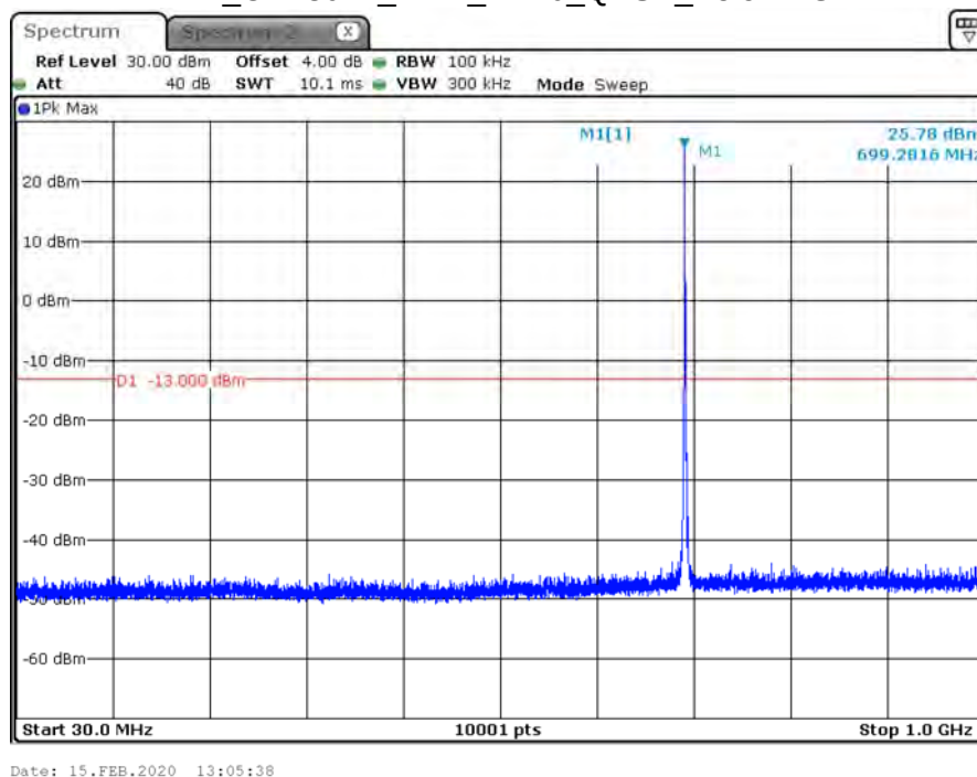
B12_CH23017_1.4M_1RB0_QPSK_Below 1G
