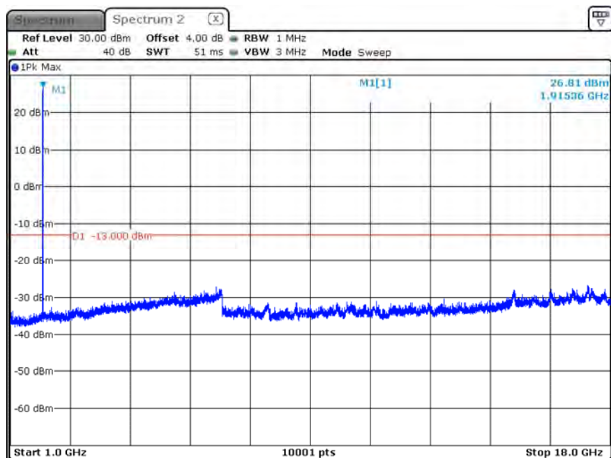
B25_CH26683_1.4M_1RB5_QPSK_Above 1G
