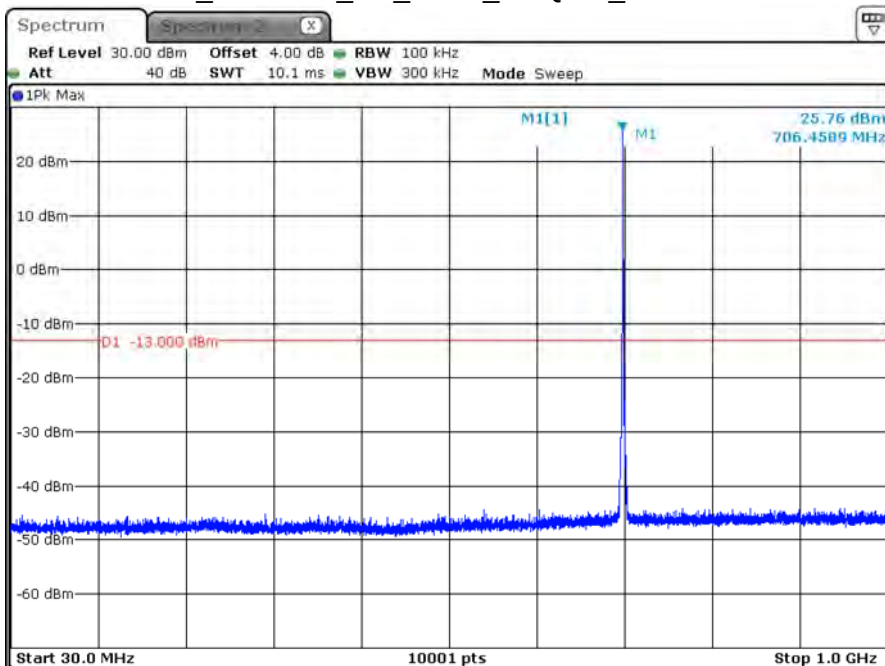
B12_CH23095_3M_1RB0_16-QAM_Below 1G
