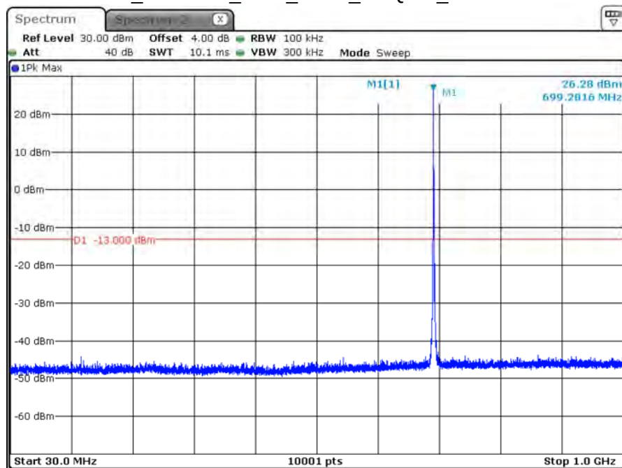
B12_CH23017_1.4M_1RB0_16-QAM_Below 1G
