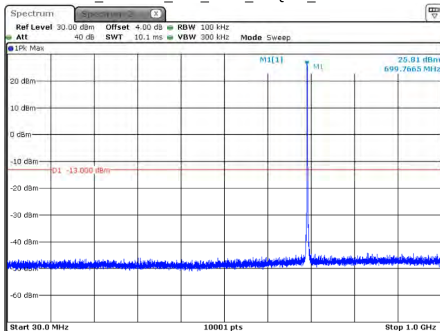
B12_CH23060_10M_1RB0_16-QAM_Below 1G
