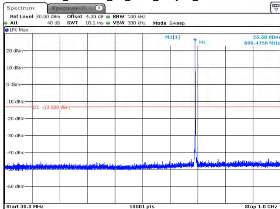
B12_CH23025_3M_1RB0_16-QAM_Below 1G
