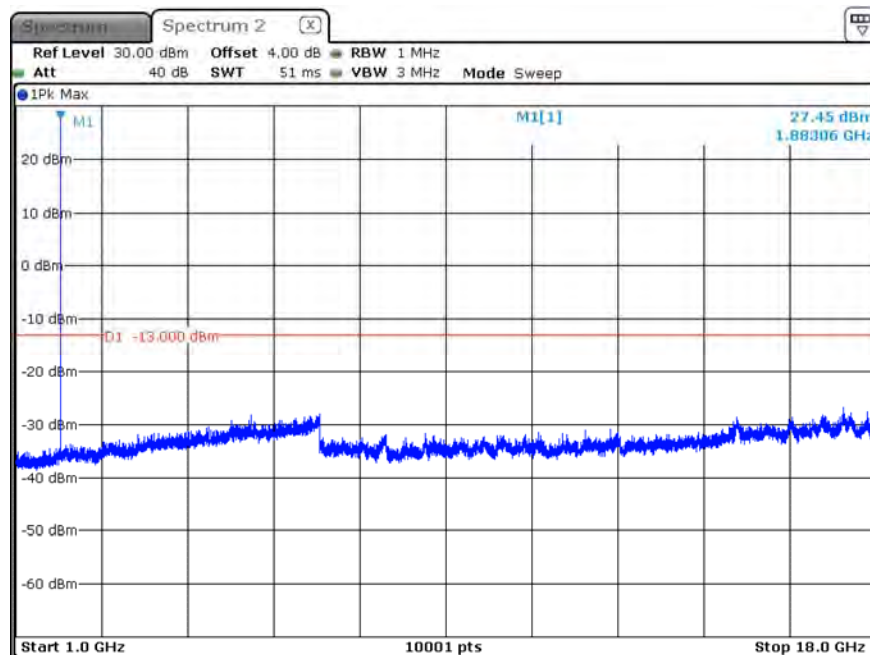
B25_CH26365_1.4M_1RB0_QPSK_Above 1G
