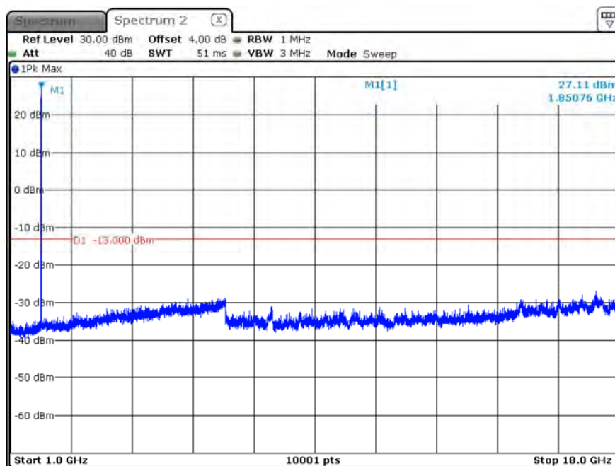
B25_CH26047_1.4M_1RB0_QPSK_Above 1G
