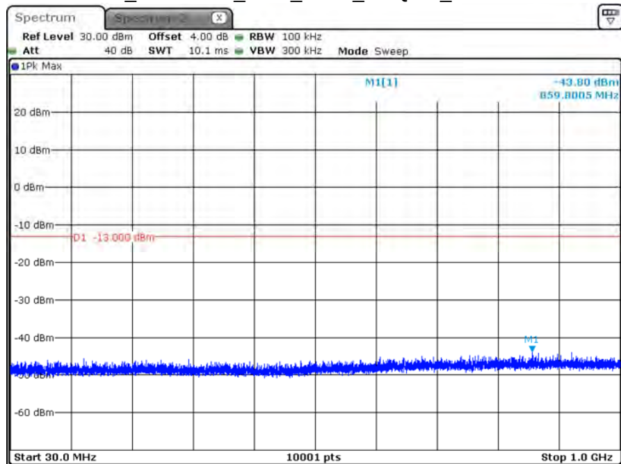
B66_CH132665_1.4M_1RB5_16-QAM_Below 1G
