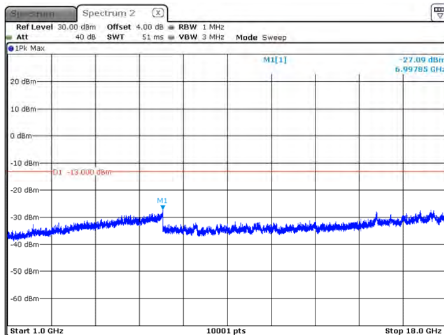
B12_CH23095_1.4M_1RB0_16-QAM_Above 1G
