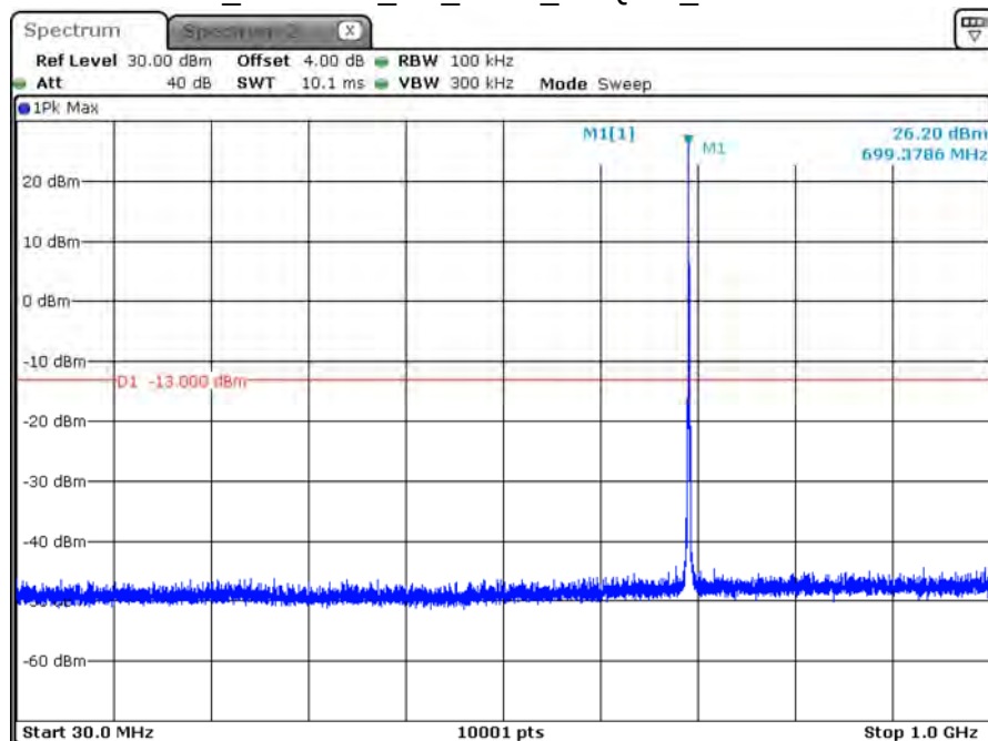
B12_CH23035_5M_1RB0_16-QAM_Below 1G
