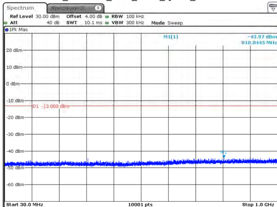
B25_CH26365_1.4M_1RB0_QPSK_Below 1G
