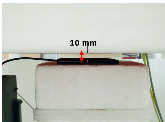
Fig.4 EUT Front side to flat phantom
