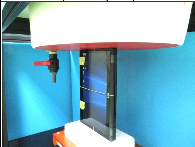
Right Side of EUT with 0 cm Gap (Tablet_Body Mode)
