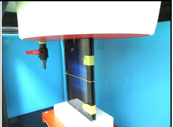
Left Side of EUT with 0 cm Gap (Tablet_Body Mode)
