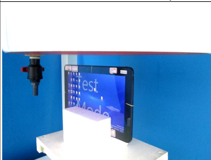
Top Side of EUT with 2.6 cm Gap
