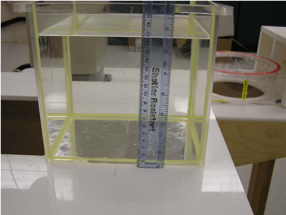
Photo2: Photo to demonstrate 15 cm Z-axis flat phantom
