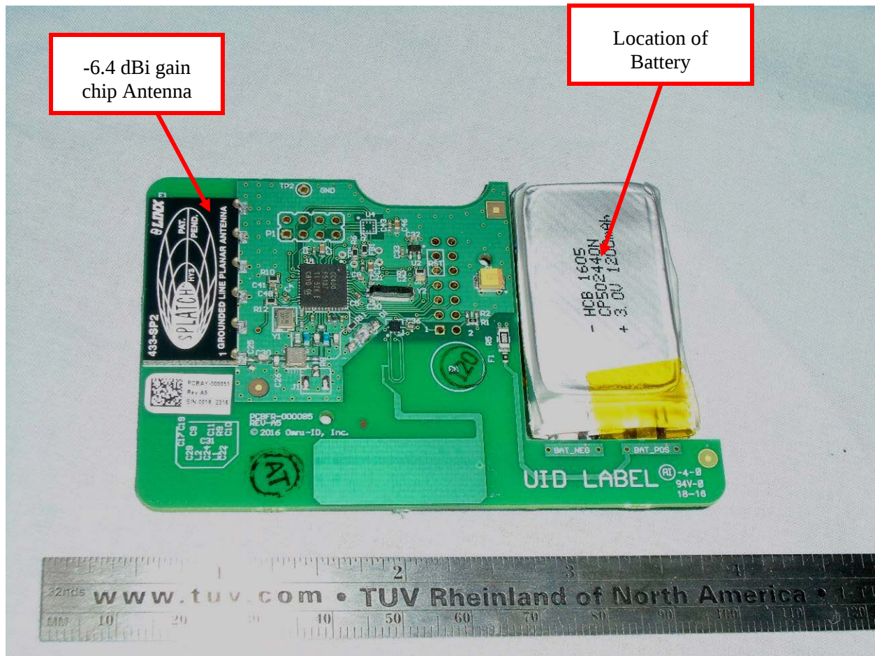
Figure 2: Top View of PCB showing the ANT-433-SP chip antenna.
