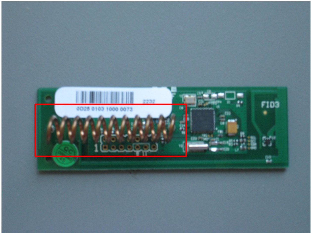
Component Side Internal Photograph – Coil Antenna Shown inside Red Box
