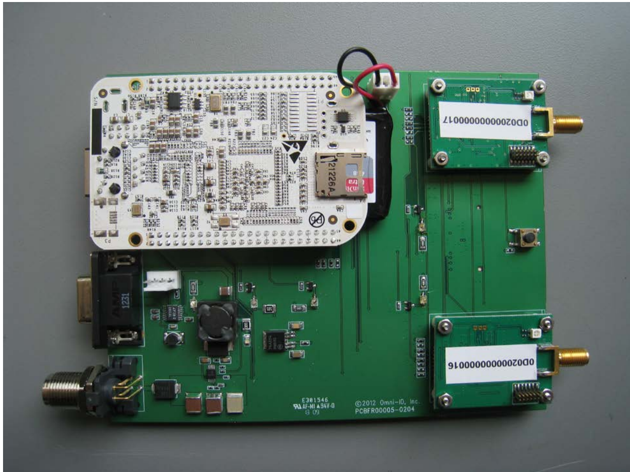
Top Side Internal Photograph
