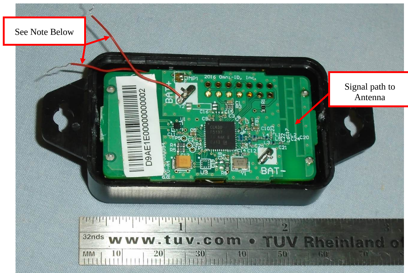
Figure 1: Bottom view of EUT with case back Removed.
