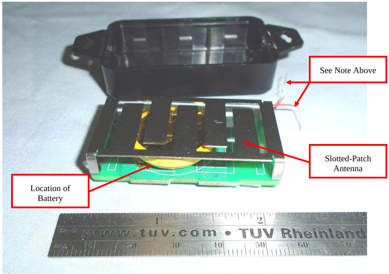
Figure 2: Top View of PCB showing the Slotted-Patch antenna.
