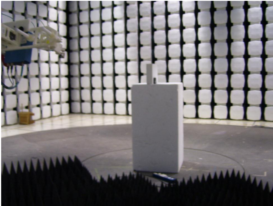
Figure 4: Above 1000 MHz
