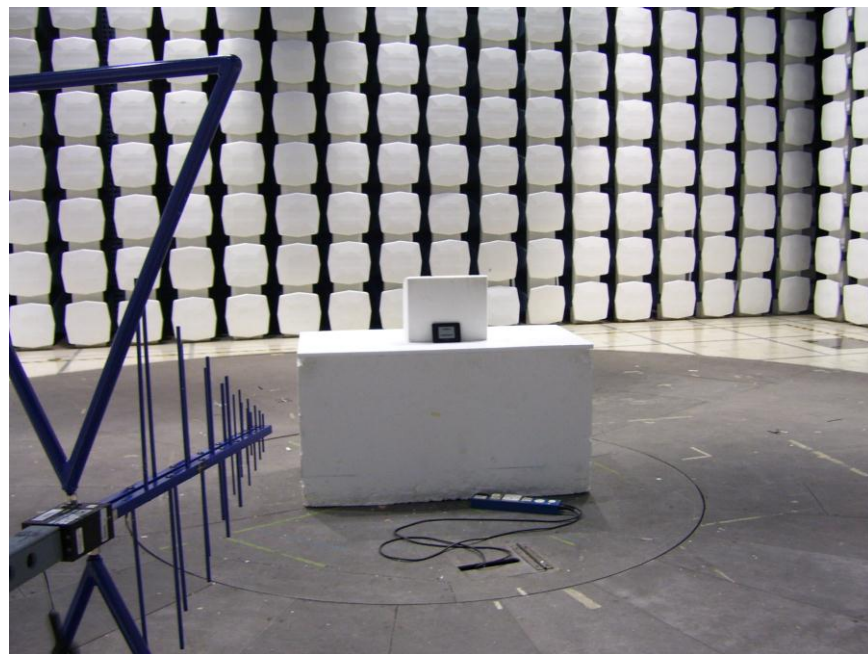
Figure 2: Radiated Emissions
