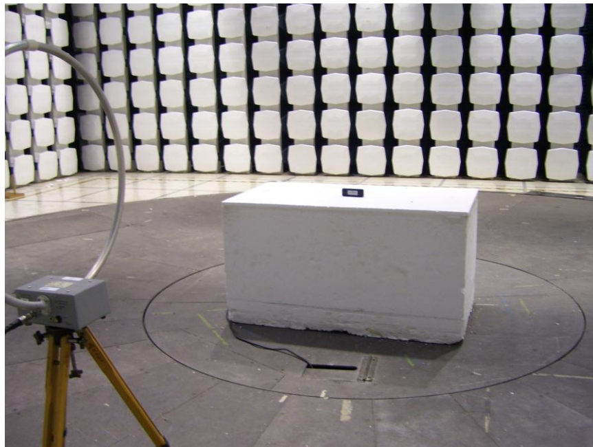
Figure 6: 9 kHz to 30 MHz
