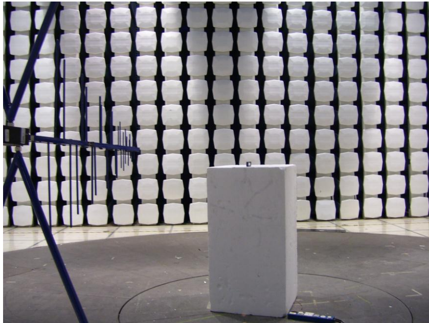
Figure 3: Radiated Emissions C63.10:2013
