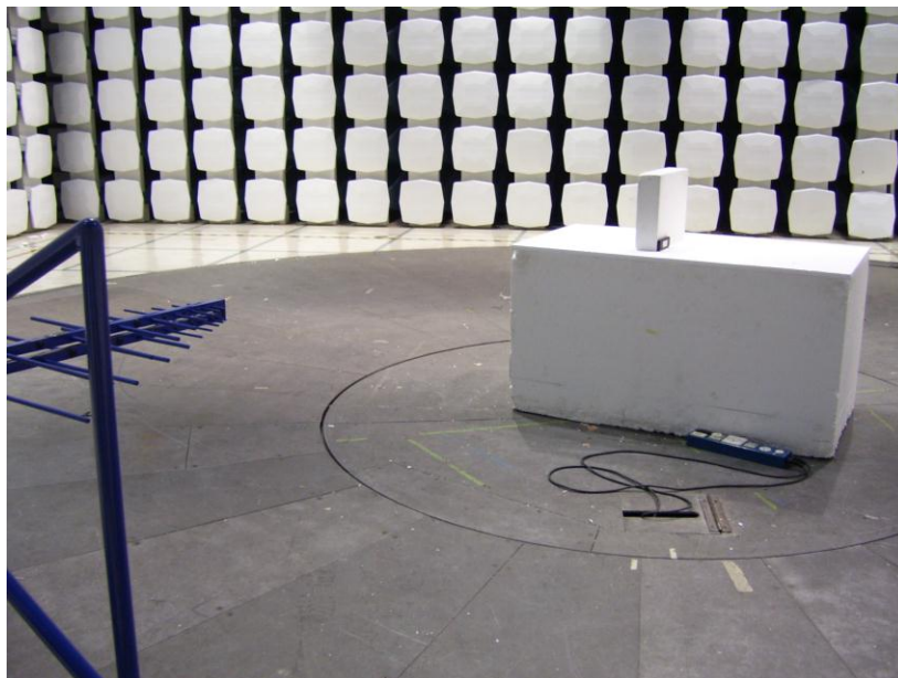
Figure 2: Radiated Emissions
