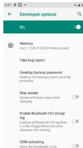
Figure 7-36 Developer Option
