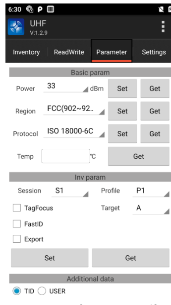
Figure 8-10 Hardware Settings
