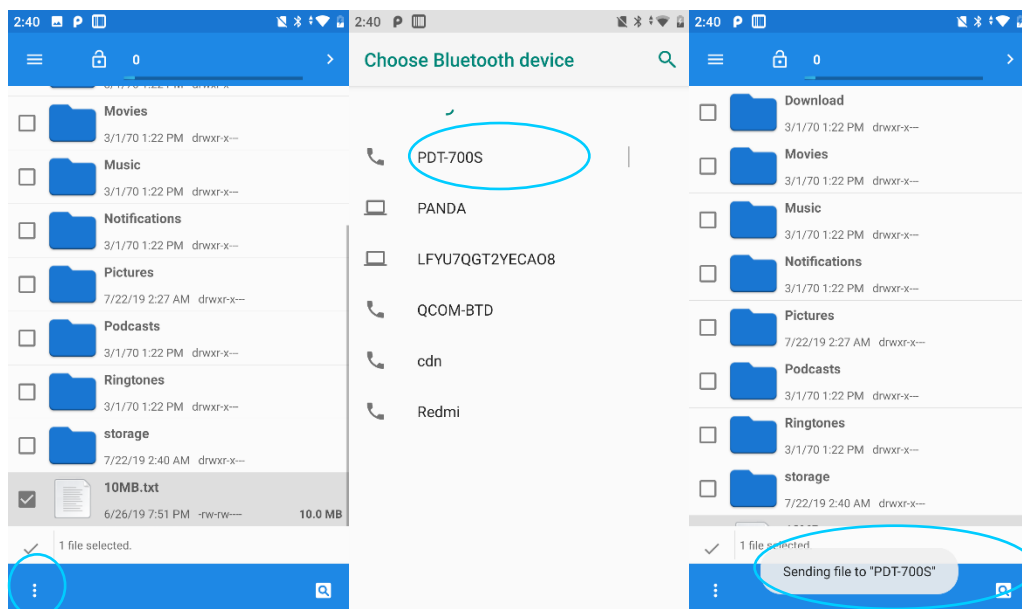
Figure 7-5 Bluetooth Transmission
