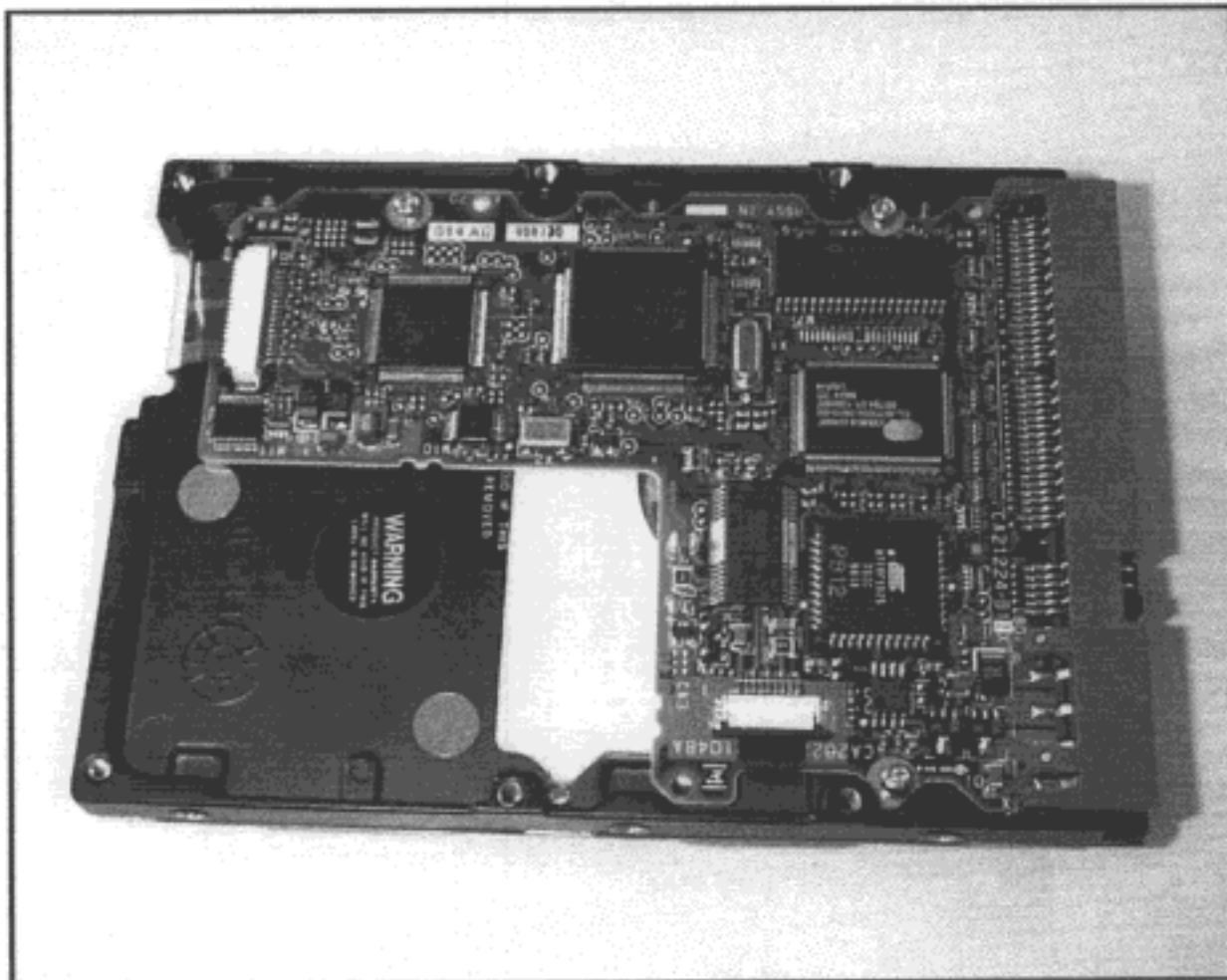
HARD DISK MOTHER BOARD COMPONENT SIDE VIEW
