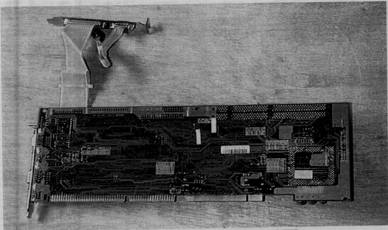
7.6..CPU BOARD SOLDER SIDE VIEW
