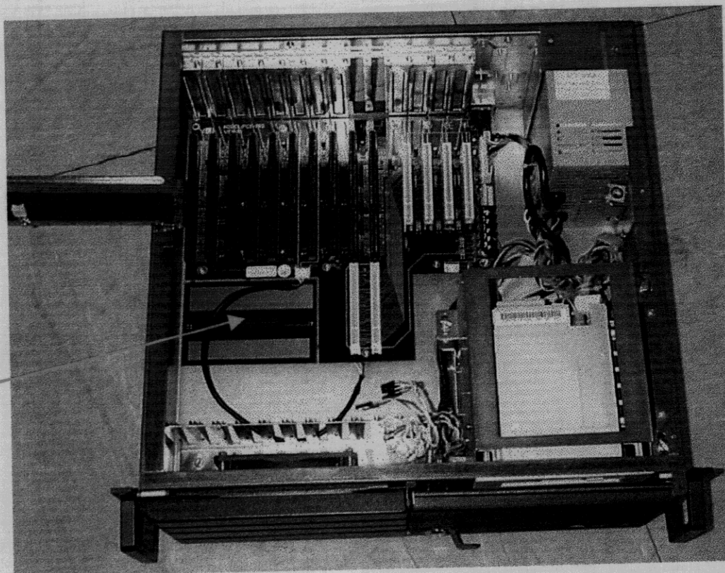
7.4.INTERNAL VIEW SHOWING THE PASSIVE RISER CARD
