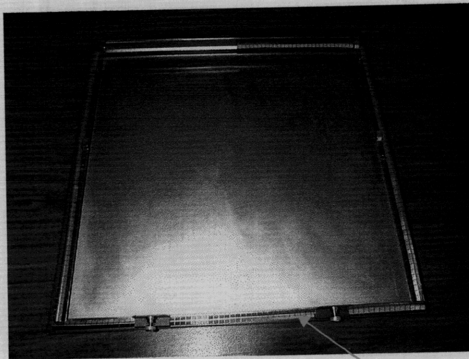
7.2.. TOP COVER VIEW SHOWING THE SHIELDING SPRINGS
