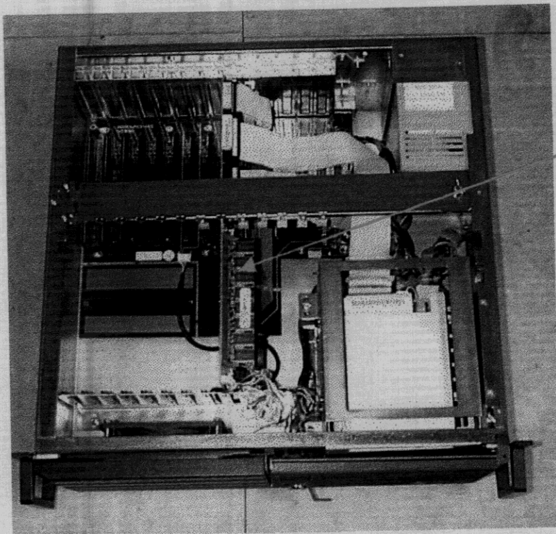
7.3.INTERNAL VIEW SHOWING THE CPU BAORD MOUNTED ONTHE PASSIVE RISER CARD
