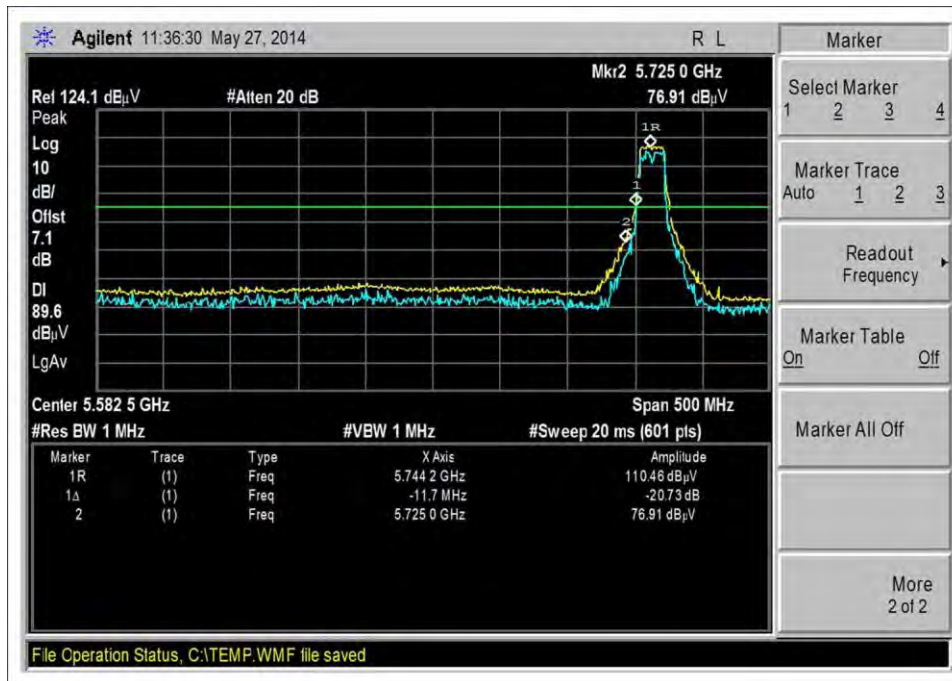
11dbi ant_11n-20_13.5dbm_5745MHz
