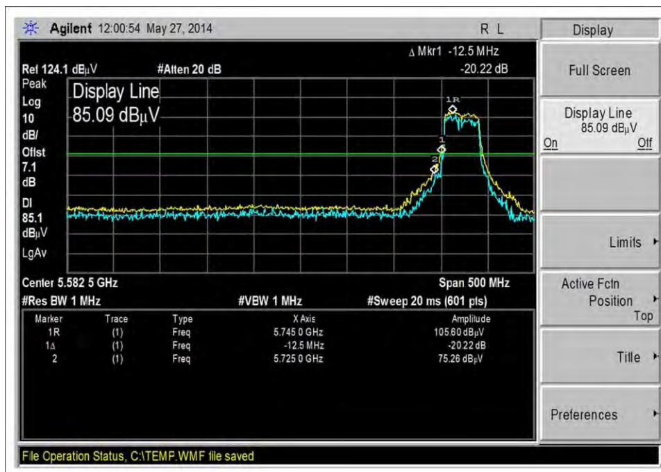
11dbi ant_11n-40_11dbm_5755MHz
