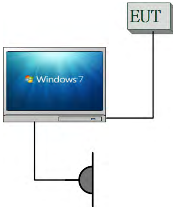
Fig. 2-2 Conducted (Antenna Port) Configuration Emission
