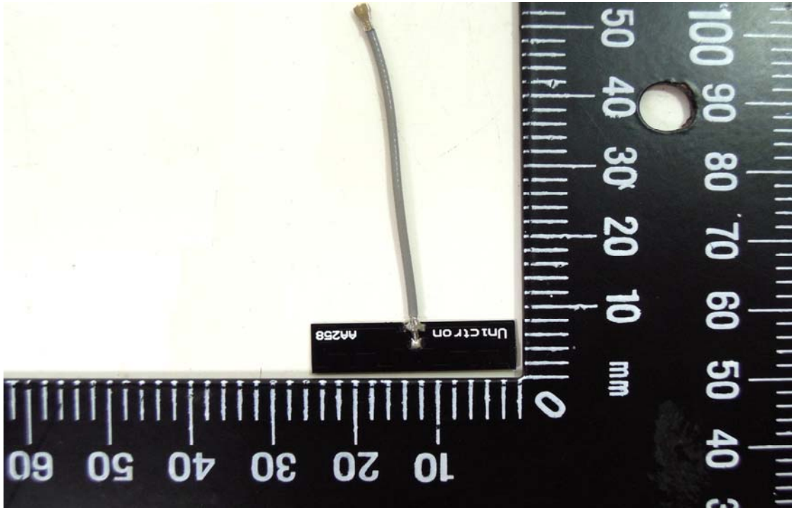
Antenna-2
