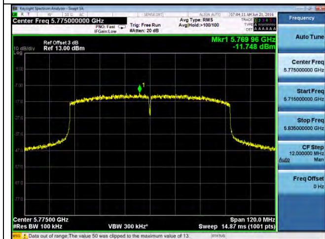
PSD-802.11ac-80M-5775M
