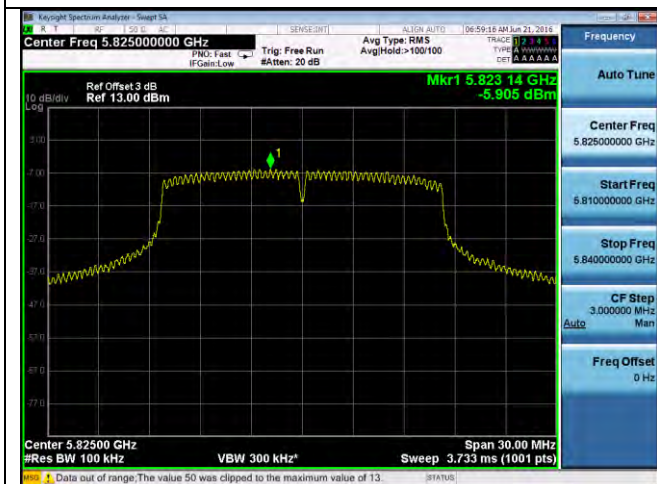
PSD-802.11a-5825M
