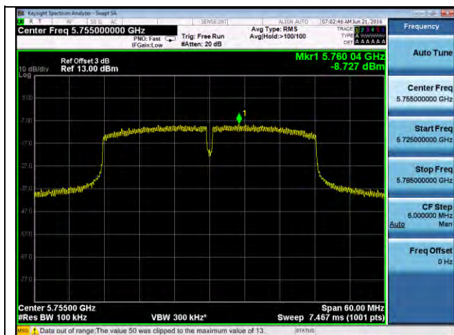
PSD-802.11n-40M-5755M
