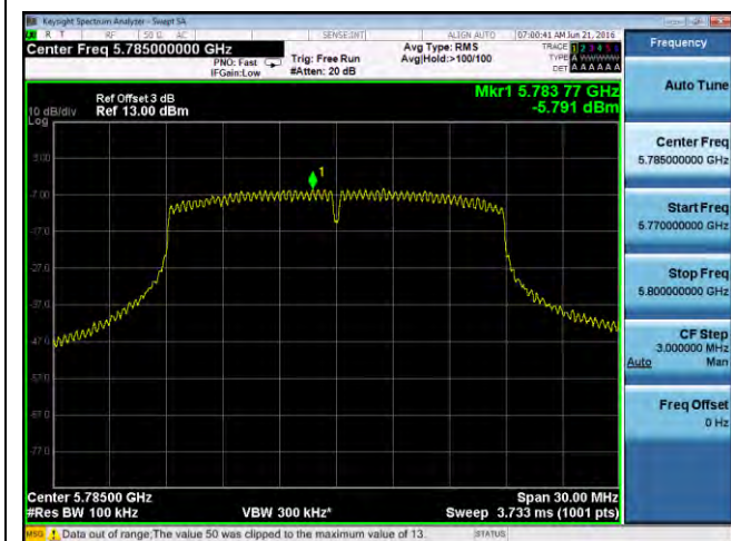
PSD-802.11n-20M -5785M
