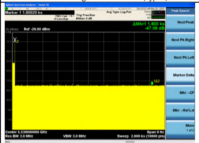
Non-Occupancy Period - 5530MHz
