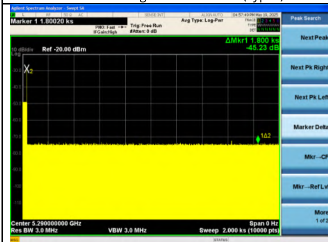
Non-Occupancy Period - 5290MHz
