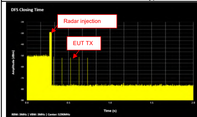
Channel Closing Time - 5290MHz (Type0)
