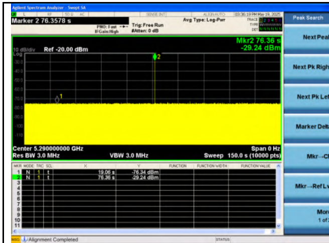
Radar at end of CAC - 5290MHz
