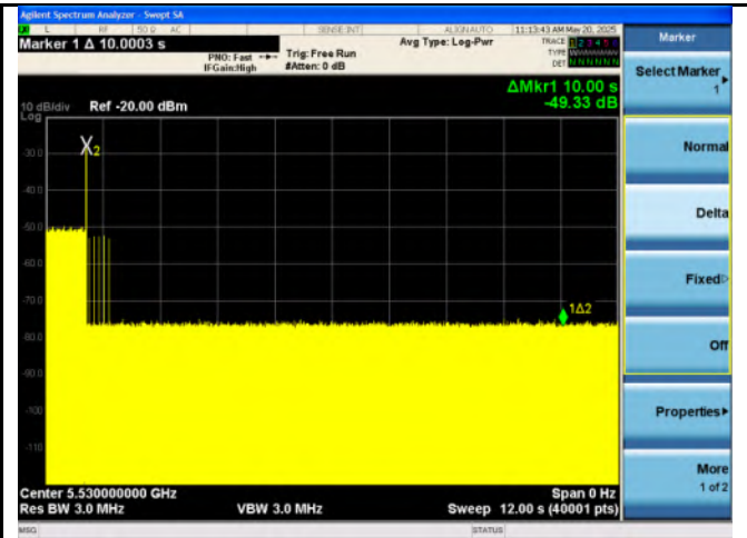
Channel Move Time - 5530MHz (Type0)
