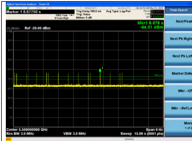
Radar Type 5
