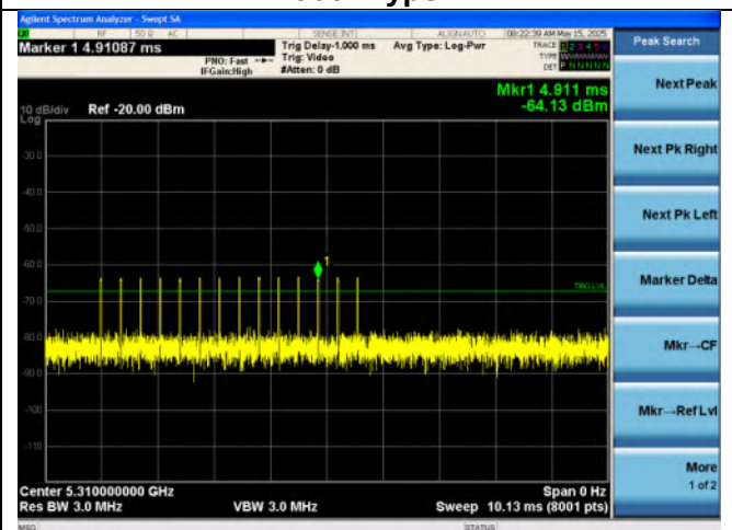
Radar Type 4
