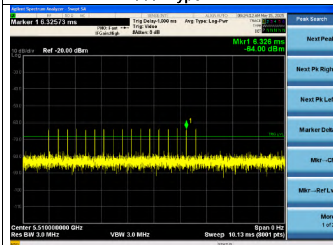
Radar Type 3
