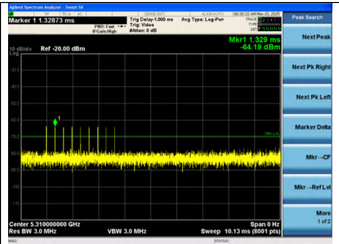
Radar Type 6
