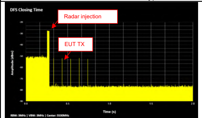
Channel Closing Time - 5530MHz (Type0)
