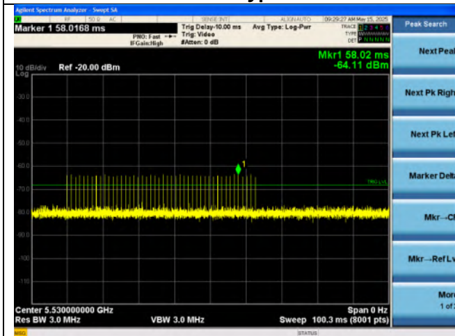
Radar Type 1B
