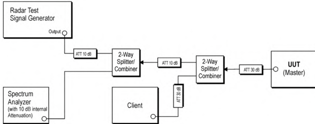
Test Setup Block Diagram
