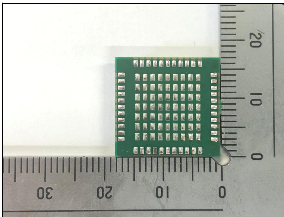
Bottom view
