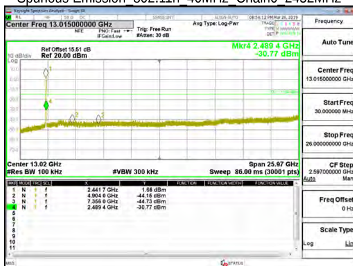
Spurious Emission 802.11n 40MHz Chain0 2452MHz
