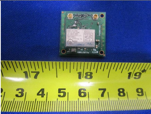
Radio Module - Top View
