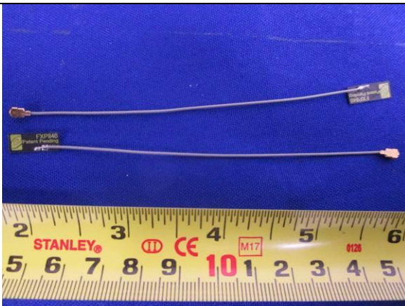
Taoglas FXP840.07.0055B Monopole Antenna- Top View
