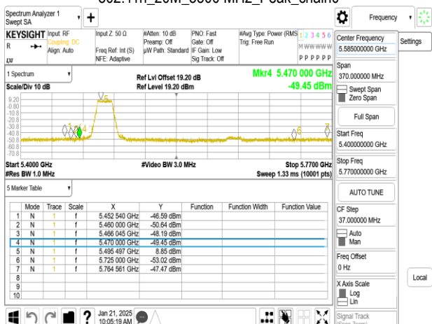
802.11n_20M_5500 MHz_Peak_chain1
