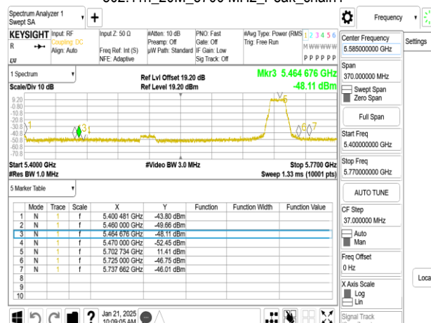
802.11n_20M_5700 MHz_Peak_chain1
