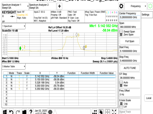
802.11n 40M_5310 MHz_Avg_chain0
