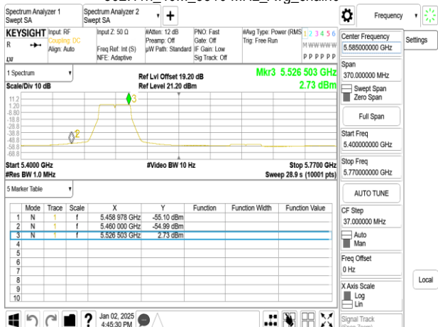
802.11n_40M_5510 MHz_Avg_chain1
