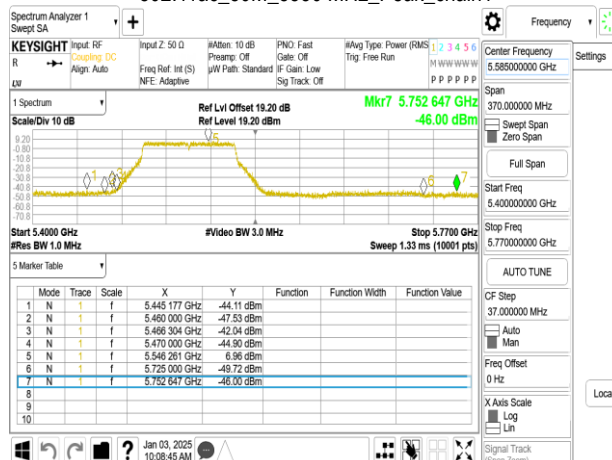
802.11ac_80M_5530 MHz_Avg_chain0
