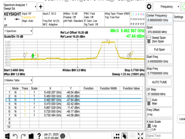
802.11n_40M_5710 MHz_Peak_chain0
