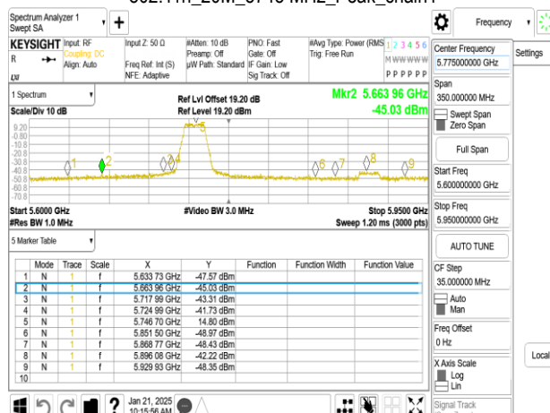
802.11n_20M_5745 MHz_Peak_chain1
