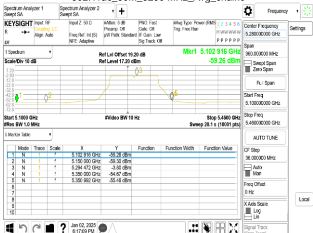
802.11ac_80M_5290 MHz_Avg_chain1
