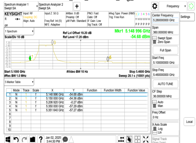
802.11n_40M_5190 MHz_Avg_chain1
