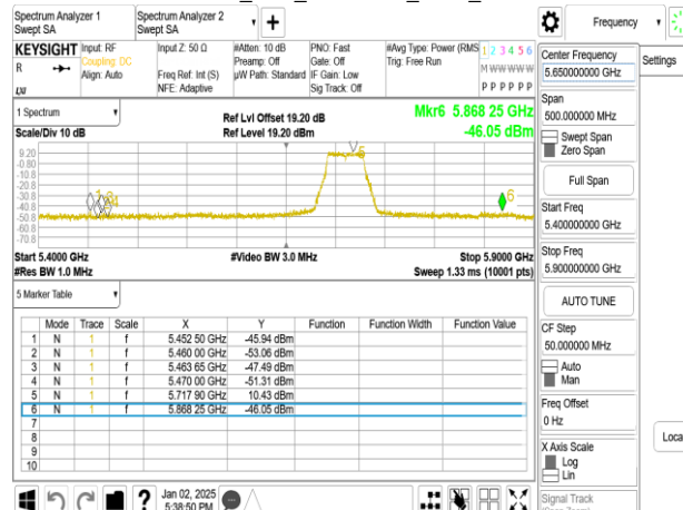
802.11n_40M_5710 MHz_Peak_chain1
