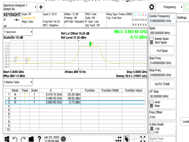
802.11ac_80M_5690 MHz_Avg_chain1
