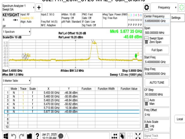
802.11n_20M_5720 MHz_Peak_chain1
