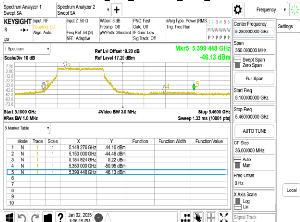
802.11ac_80M_5210 MHz_Avg_chain0
