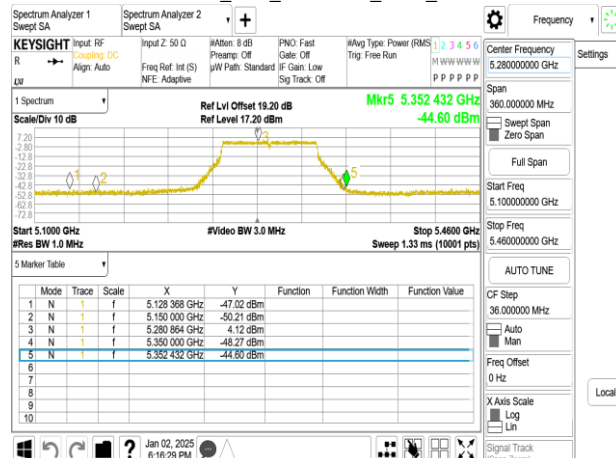
802.11ac_80M_5290 MHz_Peak_chain1
