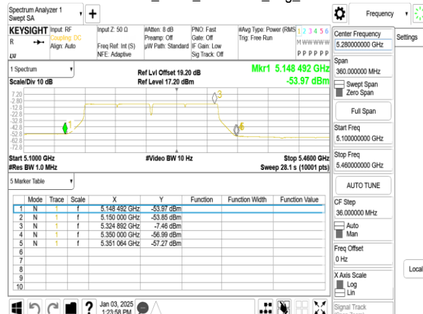
802.11ac_160M_5250 MHz_Avg_chain1
