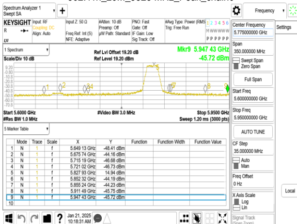
802.11n_20M_5825 MHz_Peak_chain1
