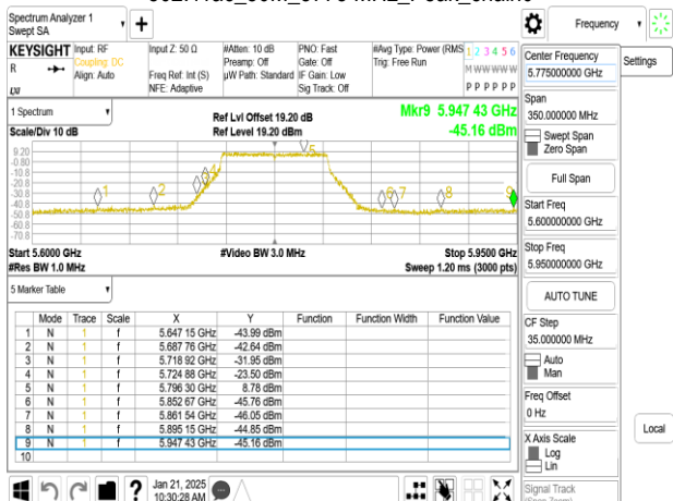
802.11ac_80M_5775 MHz_Peak_chain1
