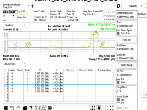
802.11n_20M_5700 MHz_Peak_chain1
