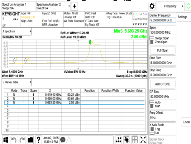
802.11n_40M_5710 MHz_Avg_chain1
