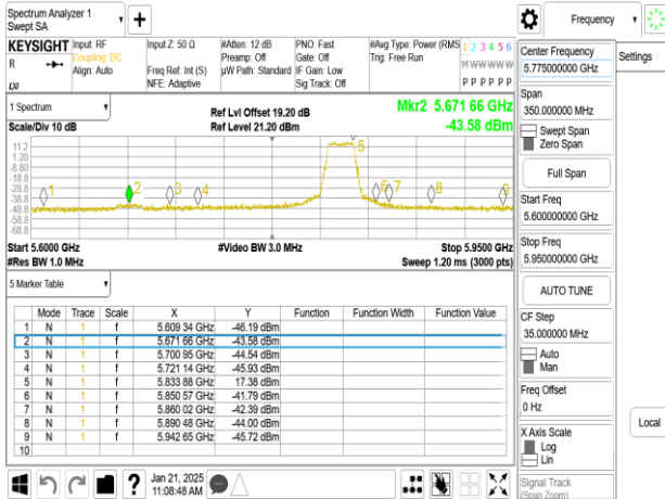
802.11be_20M_5825 MHz_Peak_chain1
