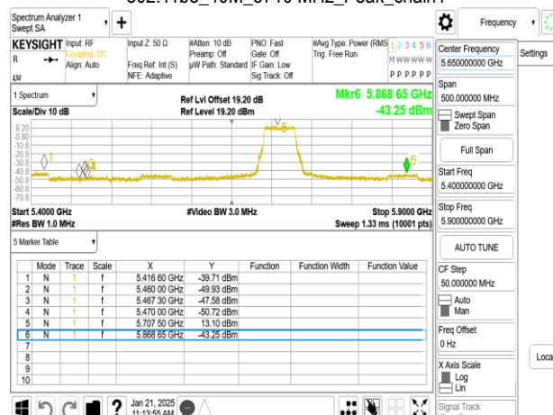
802.11be_40M_5710 MHz_Peak_chain1
