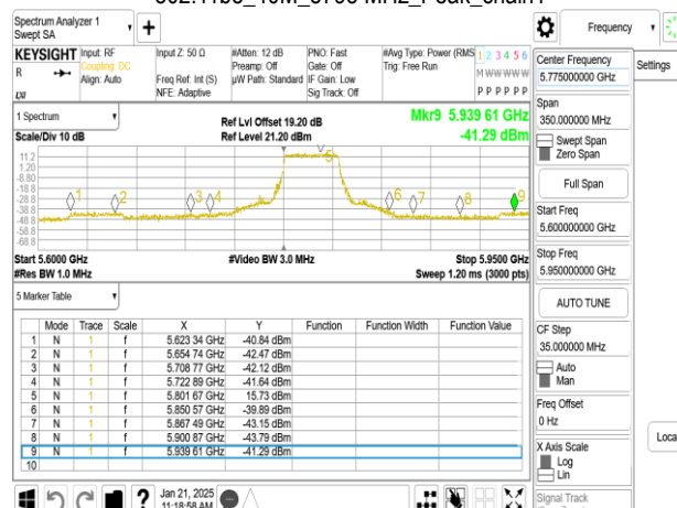
802.11be_40M_5795 MHz_Peak_chain1
