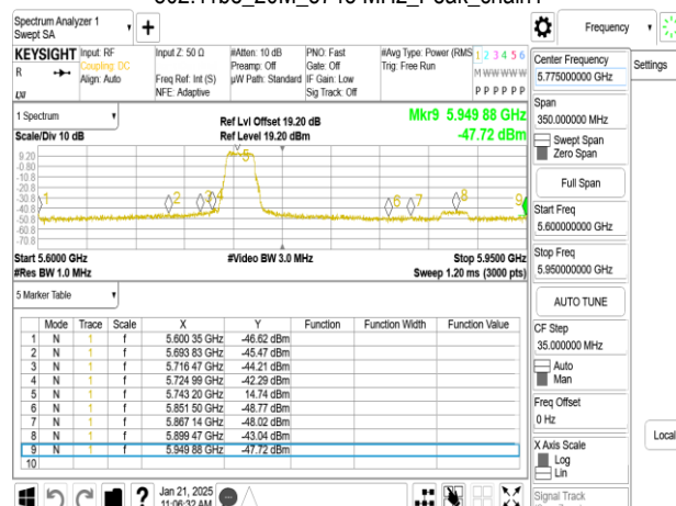
802.11be_20M_5745 MHz_Peak_chain1
