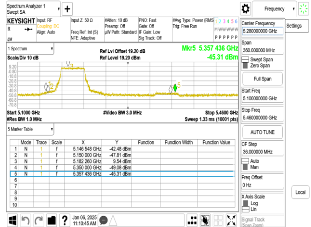
802.11be_40M_5190 MHz_Avg_chain0
