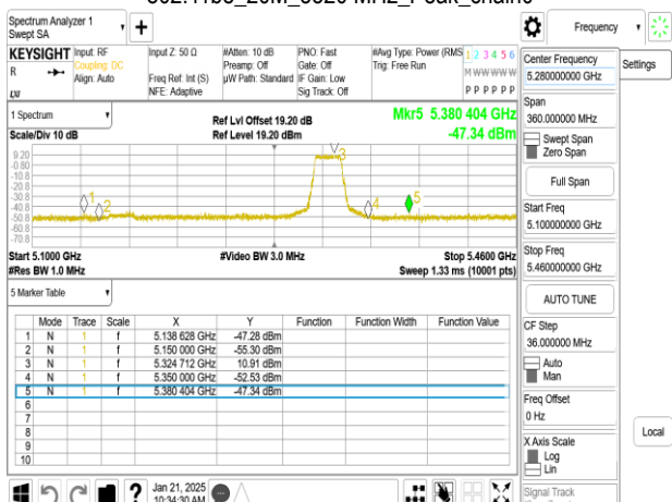
802.11be_20M_5320 MHz_Peak_chain0
