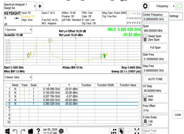
802.11be_40M_5190 MHz_Avg_chain1
