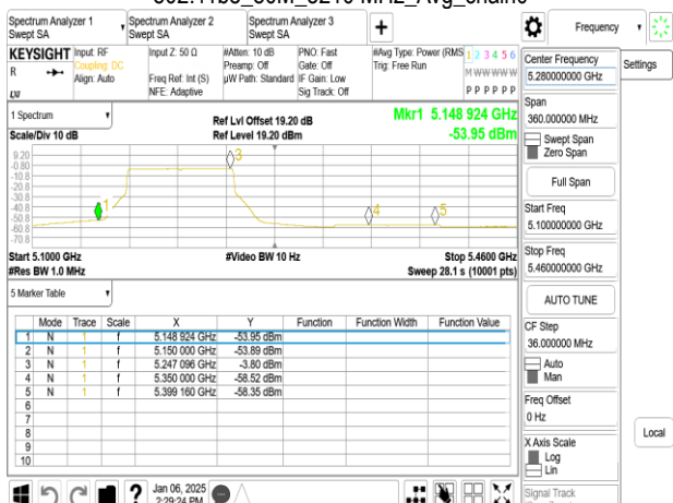
802.11be_80M_5210 MHz_Avg_chain0
