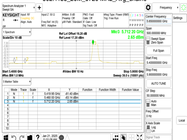
802.11be_20M_5720 MHz_Avg_chain0
