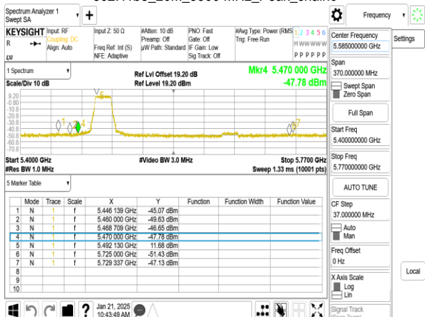
802.11be_20M_5500 MHz_Peak_chain1
