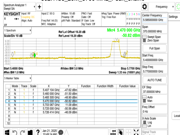
802.11be_20M_5700 MHz_Peak_chain1
