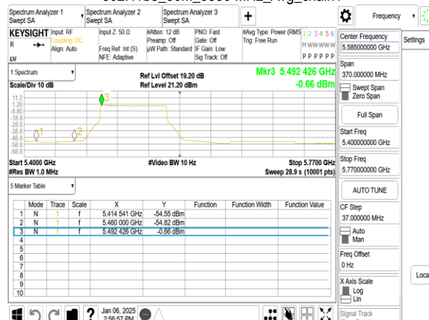
802.11be_80M_5530 MHz_Avg_chain1
