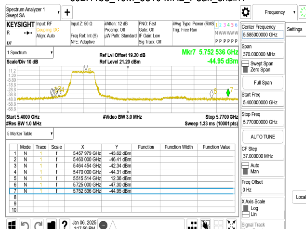
802.11be_40M_5510 MHz_Peak_chain1
