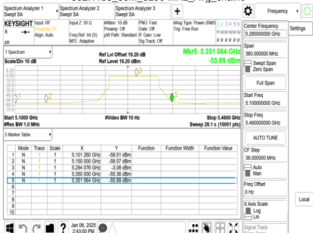
802.11be_80M_5290 MHz_Avg_chain1
