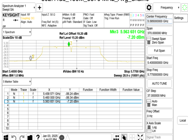
802.11ac_160M_5570 MHz_Avg_chain0
