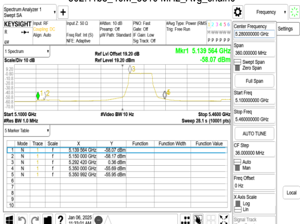
802.11be_40M_5310 MHz_Avg_chain0
