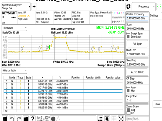
802.11be_40M_5755 MHz_Peak_chain0
