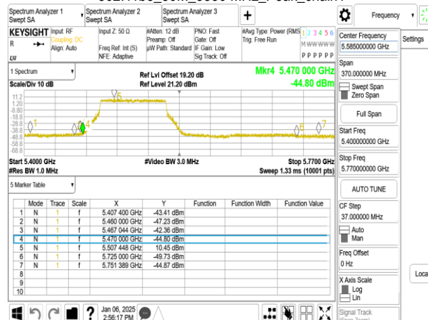
802.11be_80M_5530 MHz_Avg_chain0
