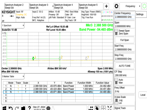
802.11g_20MHz_Chain0_2437MHz_L
