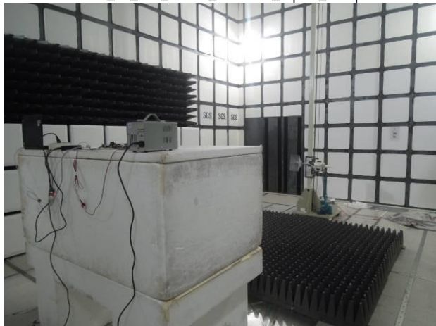
FCC_15_247_WLAN_Radiated_Dipole_Setup
