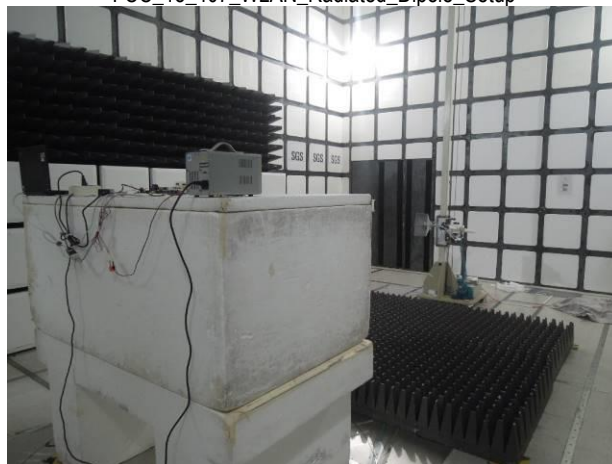
FCC_15_407_WLAN_Radiated_Dipole_Setup
