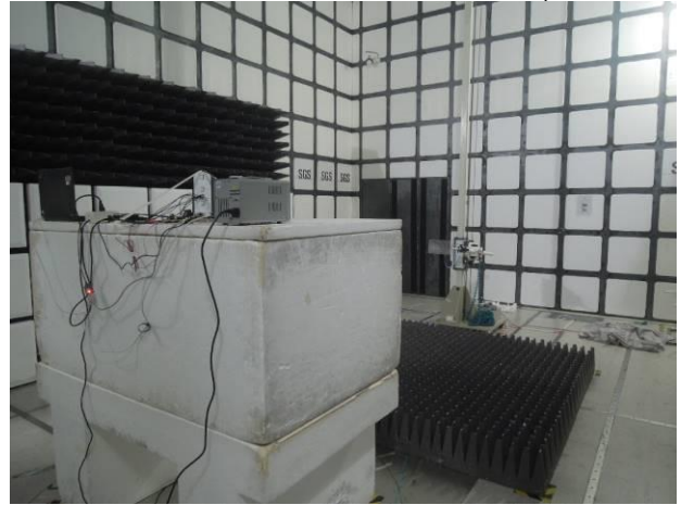
FCC_15_407_WLAN_Radiated_PIFA_Setup
