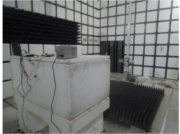
FCC_15_247_WLAN_Radiated_Monopole_Setup
