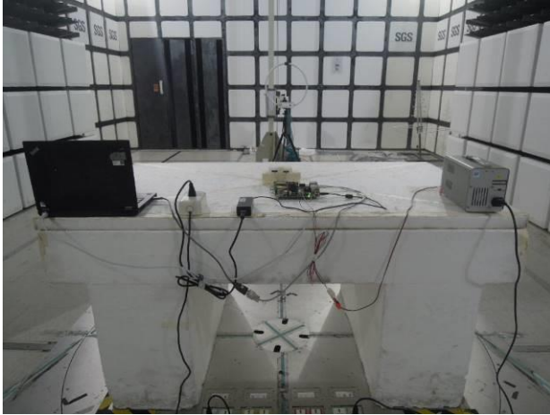
FCC_15_247_WLAN_Radiated_Monopole_Setup
