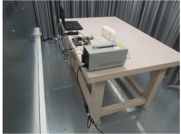
FCC_15_407_WLAN_Conduction_Setup
