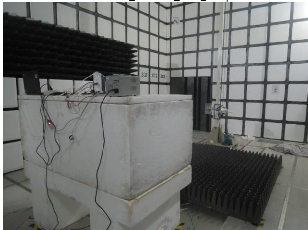
Co-location_Radiated_PIFA_Setup
