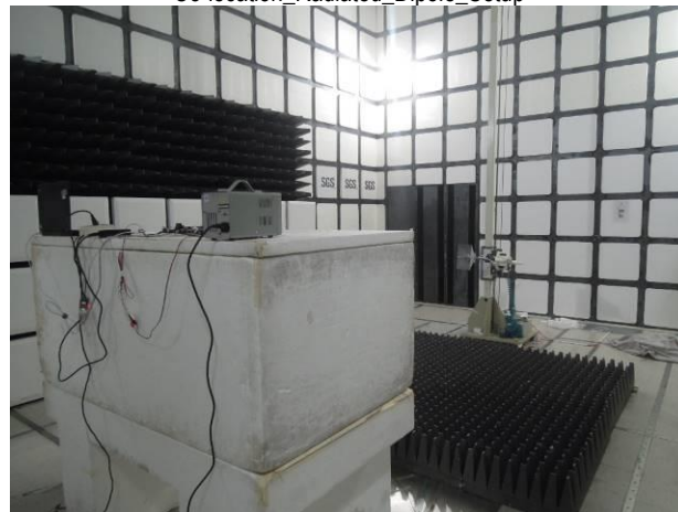
Co-location Radiated Dipole Setup
