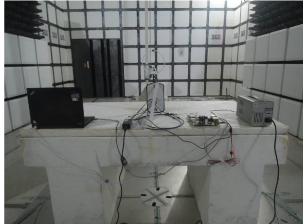
FCC_15_407_WLAN_Radiated_PIFA_Setup
