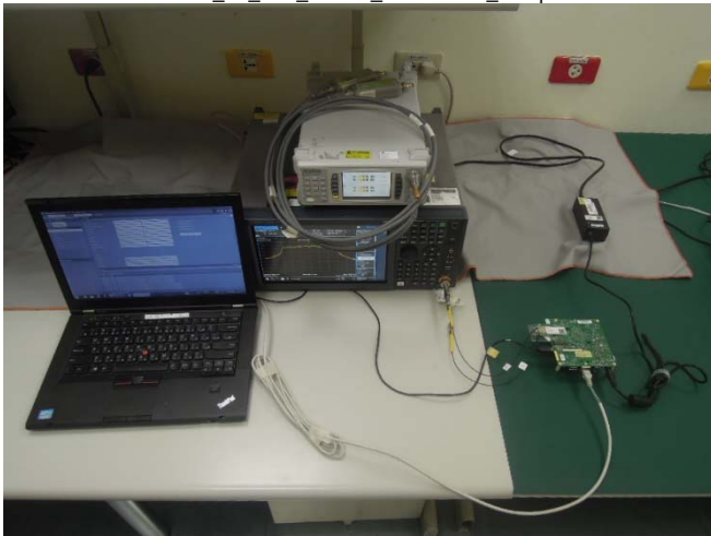
FCC_15_407_WLAN_Radiated_Setup_Monopole antenna (GW.05.0153)
