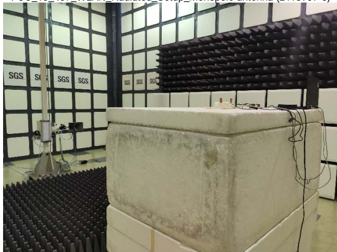
FCC_15_407_WLAN_Radiated_Setup_Monopole antenna (2118907-8)
