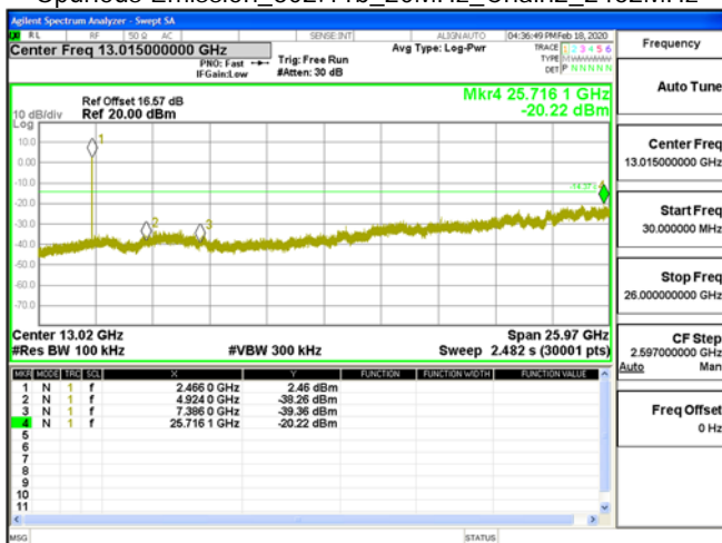
Spurious Emission_802.11b_20MHz_Chain2_2462MHz
