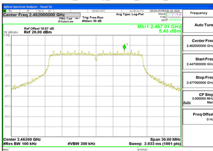
Reference Level_802.11g_20MHz_Chain2_2462MHz
