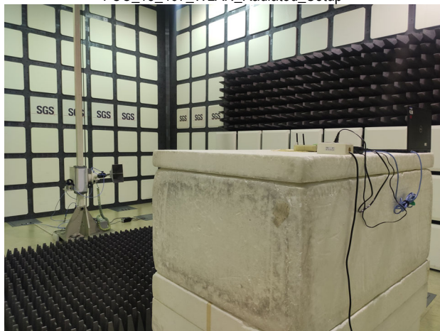
FCC_15_407_WLAN_Radiated_Setup
