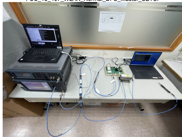
FCC_15_407_WLAN_Normal_DFS_Master_SETUP
