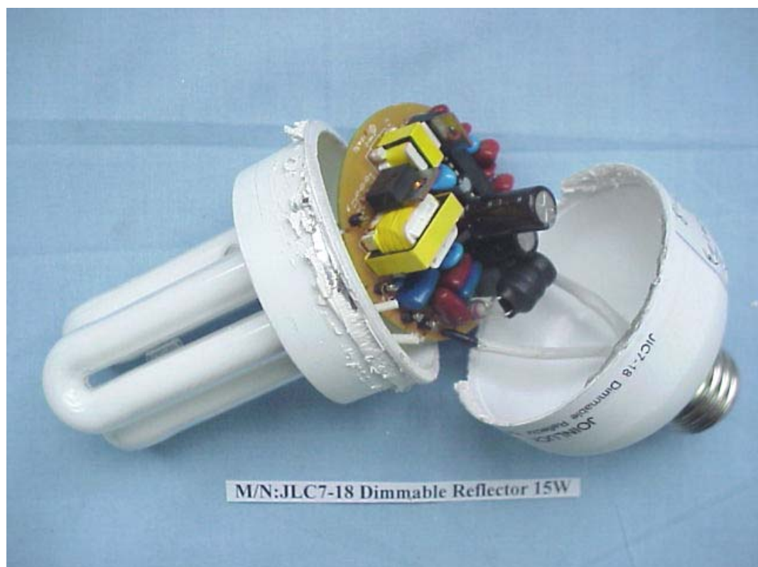
FIGURE 2 ENERGY SAVING LAMP (M/N: JLC7-18 DIMMABLE REFLECTOR 15W) COVER REMOVED 2
