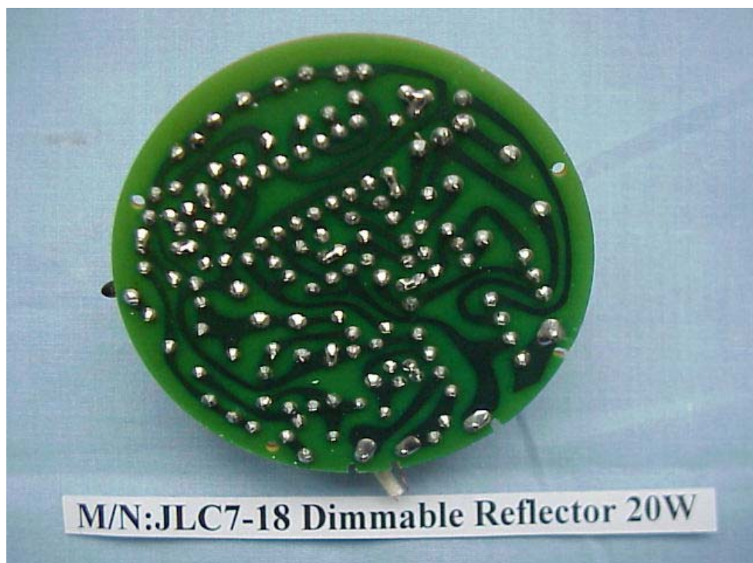
FIGURE 8 ENERGY SAVING LAMP (M/N: JLC7-18 DIMMABLE REFLECTOR 20W) MAIN BOARD (SOLDERED SIDE)
