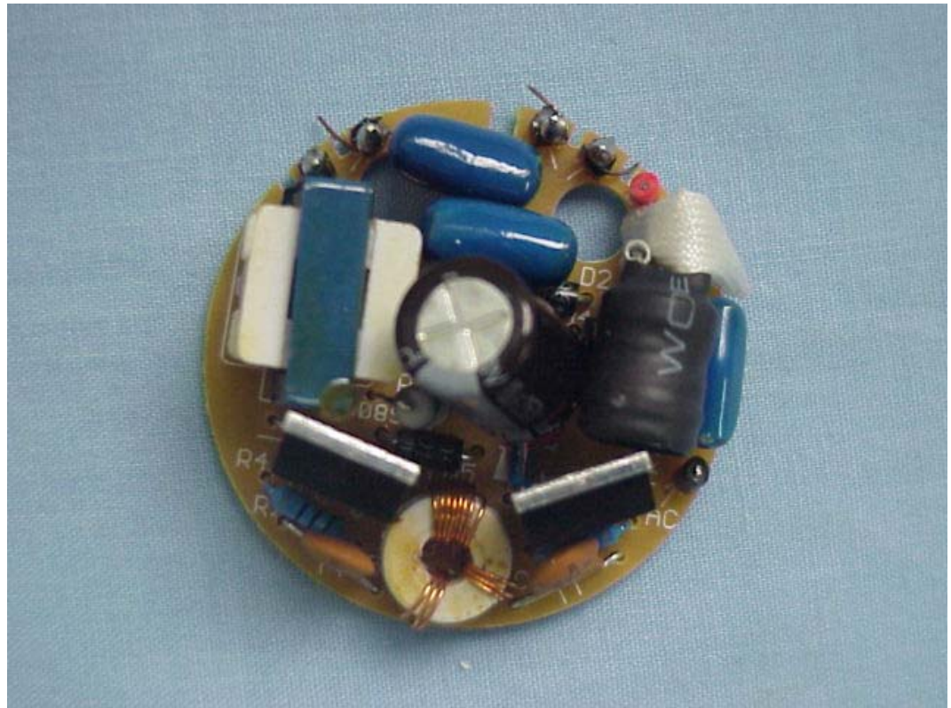
FIGURE 2 ELECTRONIC ENERGY SAVING LAMP (M/N: JLC7-18 A-TYPE 9W) MAIN BOARD (COMPONENT SIDE)
