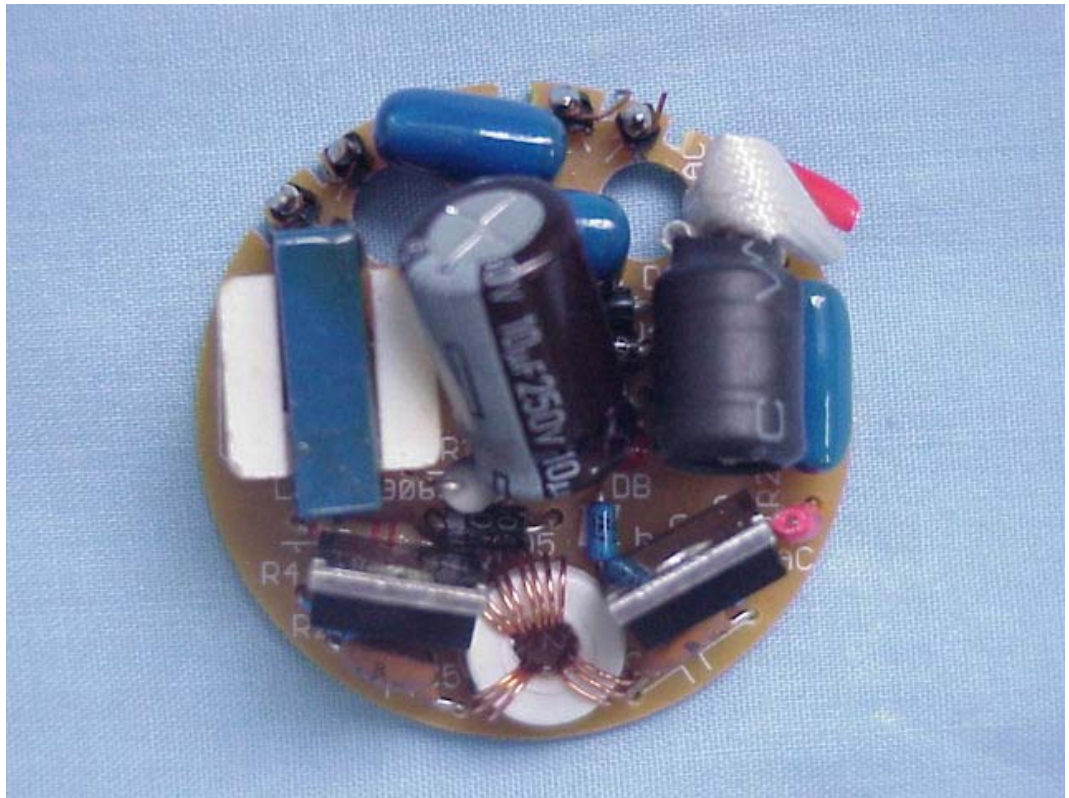
FIGURE 5 ELECTRONIC ENERGY SAVING LAMP (M/N: JLC7-18 GLOBE 9W) MAIN BOARD (COMPONENT SIDE)
