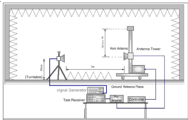
Figure 4. above 1GHz
